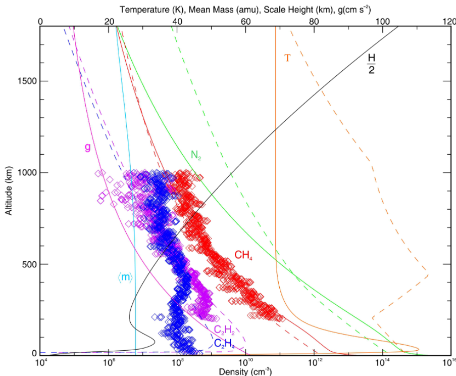
Fig. 3. Pluto's atmospheric composition and structure. Model profiles of temperatures, densities, and other relevant quantities (such as gravity g , mean mass \bar{m} , and \text{N}_2 density scale height H —plotted as H/2 in order to facilitate a common x axis range) in the atmosphere of Pluto are shown, which are consistent with the transmission results of Fig. 2. Methane, acetylene, and ethylene densities retrieved from the solar occultation data are indicated (diamonds). Pre-encounter model values (37) are given by dashed lines. Pluto's upper atmosphere is very cold ( T \sim 70 K), resulting in a very low escape rate.
