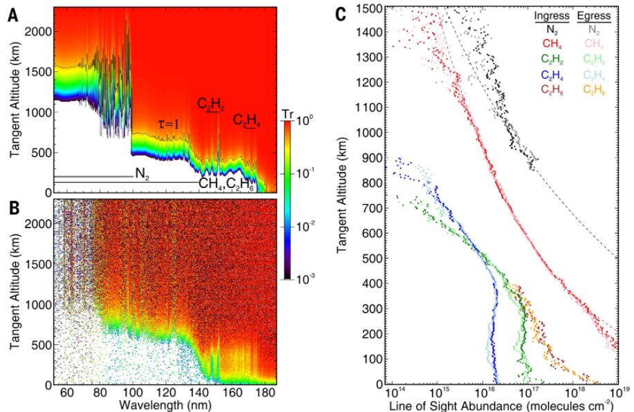
Fig. 2. Ultraviolet transmission of Pluto’s atmosphere. (A) Line-of-sight (LOS) transmission as a function of ultraviolet wavelength and tangent altitude for the M2 model Pluto atmosphere (37), with the \tau = 1 line indicated along with the regions where \text{N}_2 , \text{CH}_4 , \text{C}_2\text{H}_2 , \text{C}_2\text{H}_4 , and \text{C}_2\text{H}_6 contribute to the opacity. \text{N}_2 absorbs in discrete bands for wavelengths 80 to 100 nm, with bands and an underlying continuum at wavelengths 65 to 80 nm and an ionization continuum at wavelengths of <65 nm. \text{CH}_4 dominates the opacity at wavelengths of <140 nm. \text{C}_2\text{H}_6 has a similar cross section to \text{CH}_4 but absorbs to 145 nm, where it contributes to the opacity. \text{C}_2\text{H}_2 has strong absorption bands at 144, 148, and 152 nm. \text{C}_2\text{H}_4 dominates the opacity at 155 to 175 nm. The model also contains \text{C}_4\text{H}_2 , which accounts for much of the opacity at wavelengths 155 to 165 nm. (B) LOS transmission of Pluto’s atmosphere determined from the Alice solar occultation data. The Alice data are normalized (at each ultraviolet wavelength) to unabsorbed levels at high altitude. In comparison with the model transmission, \text{N}_2 opacity begins at much lower altitudes (~500 km lower), whereas \text{CH}_4 opacity begins ~100 km higher than in the model. Pluto’s atmosphere has somewhat less \text{C}_2\text{H}_2 and \text{C}_2\text{H}_4 than the model. Continuum absorption by Pluto’s haze (not included in the model) is important at wavelengths >175 nm. (C) LOS column density profiles retrieved from the observed transmission data of (B) using known absorption cross sections for the indicated species. The quality of the data can be judged by the overlap of ingress and egress profiles (because the atmosphere is expected to be nearly spherically symmetric away from the surface) and by the amount of scatter in the data points. The dashed lines are LOS column densities computed by using the \text{N}_2 and \text{CH}_4 number density profiles in Fig. 3.
