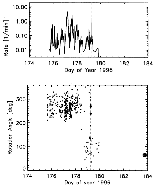
Figure 2. Dust data obtained during the first Ganymede flyby (27 June 1996). Closest approach (CA) to Ganymede is indicated by a dashed line. Upper panel: impact rate of small dust particles (ion collector charge Q_I < 10^{-13} C). Shortly after CA high noise rate caused deadtime which significantly reduced the number of recorded impacts. Note the ten hour periodicity in the impact rate. Lower panel: sensor direction at time of dust particle impact for those impacts for which complete information was available on the ground. The symbol sizes indicate the different impact charges (smallest symbols: Q_I < 10^{-13} C; for the larger dots the impact charges are Q_I \sim 10^{-13} C and \sim 10^{-11} C, respectively.) At 0^\circ the sensor points close to the ecliptic North direction, at 90^\circ and 270^\circ the sensor points close to Jupiter's equatorial plane.
