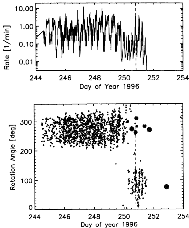
Figure 3. Same as Fig. 2, but for the second Ganymede flyby on 6 Sept 1996. Due to a different instrument configuration, deadtime did not affect the recording of dust impacts in the inner Jovian system. The reduced impact rate about one day after Ganymede CA is real. The symbol sizes in the lower panel represent 4 orders of magnitude of impact charge.
