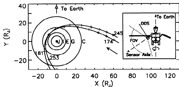
Figure 1. Galileo's trajectories during both Ganymede flybys projected onto Jupiter's (J) equatorial plane (Jupiter radius, R_J = 71,492 km). The orbits of the Galilean satellites are shown: Io (I), Europa (E), Ganymede (G), and Callisto (C). Dates are marked by crosses (numbers give day of year) on Galileo's paths through the Jovian system. The inset shows the spacecraft orientation: the antenna (top) points towards Earth, and the dust detector (DDS) faces the anti-Earth hemisphere. During one spin rotation of the spacecraft the sensor axis scans a cone with 110^\circ opening angle. The dust detector itself has 140^\circ field of view (FOV).
