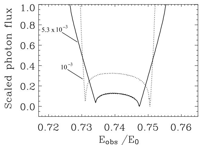
FIG. 6.—Effect on line profiles of additional broadening, such as that produced by unresolved Zeeman splitting. Shown are the observed profiles of lines with intrinsic half widths of 10^{-3} E_0 (dotted curve; the same as in the other line profile calculations reported here) and 5.3 \times 10^{-3} E_0 (solid curve; half the half width produced by rotational Doppler broadening, comparable to the splitting produced by a 10^9 G magnetic field). For each of the profiles the flux has been scaled in units of its deepest minimum. Both profiles are for R/M = 4.43 , R = 11.5 km, \nu_s = 45 Hz, i_{\text{belt}} = 90^\circ , \Delta i_{\text{belt}} = 5^\circ , isotropic emission in the frame corotating with the stellar surface, and i_{\text{spin}} = 78^\circ .
