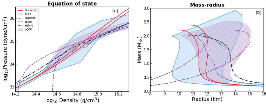
Figure 3 The pressure-density relation (EOS) (a) and the corresponding M-R relation (b) for some example models with different microphysics. Nucleonic (neutrons, protons): models AP3 and AP4 from ref. [27], also used in ref. [28]. Quark (u, d, s quarks): models from refs. [29, 30]. Hybrid (inner core of uds quarks, outer core of nucleonic matter): models from ref. [31]. Hyperon (inner core of hyperons, outer core of nucleonic matter): Model from ref. [32]. CEFT: range of nucleonic EOS based on Chiral Effective Field Theory (CEFT) from ref. [33]. pQCD: range of nucleonic EOS from ref. [34] that interpolate from CEFT at low densities and match to perturbative QCD (pQCD) calculations at higher densities than shown in this figure. All of the EOS shown are compatible with the existence of \sim 2 M_{\odot} NSs.
