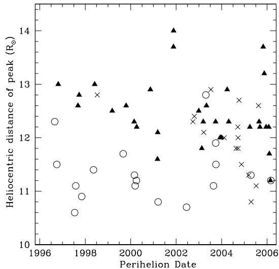
Figure 3.7: Perihelion date versus heliocentric distance of the peak magnitude for the comets observed to peak in C3. The triangles are in curve A, crosses are in curve B, and circles are in curve C.
