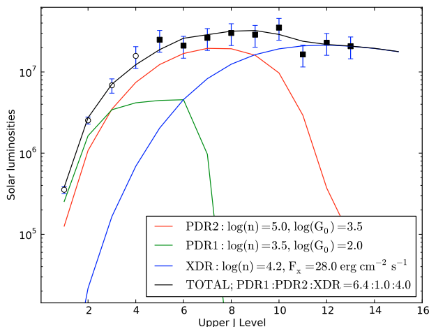
Fig. 2. Luminosities of CO lines from Mrk 231. Filled symbols represent measurements from the SPIRE FTS spectrum, while ground-based measurements are denoted with open symbols. Coloured lines indicate two model PDR components (red and green lines) and an XDR component (blue line). The sum of these three components is indicated by the black line and fits the CO measurements. In the legend, n denotes the number density of hydrogen nuclei ( n = n_{\text{H}} + 2n_{\text{H}_2} ) in \text{cm}^{-3} , G_0 denotes the incident UV flux in units of 1.6 \times 10^{-3} \text{ erg s}^{-1} \text{ cm}^{-2} for the PDRs, and F_{\text{X}} the incident X-ray flux for the XDR. The legend also indicates the relative emitting areas of the three components.
