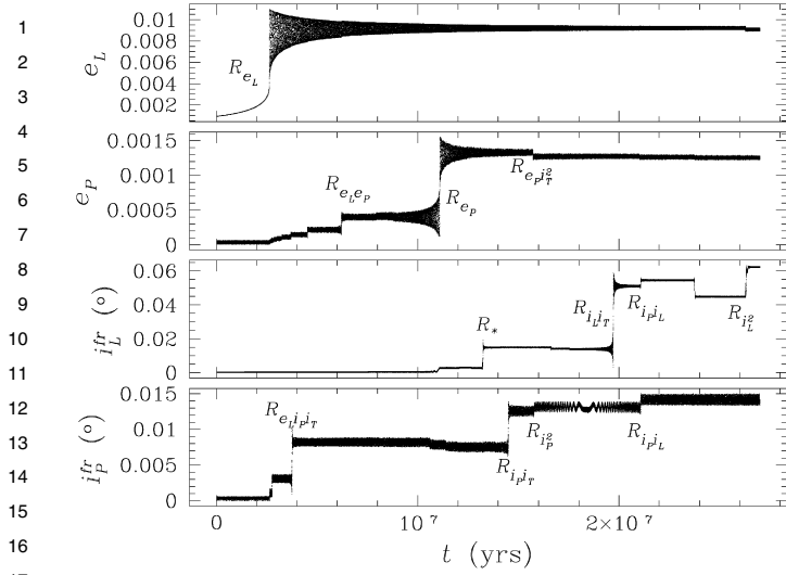
Fig. 3. The eccentricities and free inclinations of Proteus and Larissa as they diverge through the PL\ 2:1 resonances. The system consists of Neptune, Triton, and the two small satellites, started with zero free eccentricities and free inclinations. The proximity of the strong first-order R_{eL} resonance forces e_L \approx 0.001 at t = 0 ; starting close to resonance with this value is equivalent to starting with e_L = 0 at a greater distance from the resonance as actually occurs in the system. The density of the satellites is \bar{\rho} = 0.6\text{ g/cm}^3 ; a_L is fixed at 2.93R_N , while Proteus migrates outward from 4.651R_N to 4.654R_N , equivalent to Q_N = 20,000 . The strongest first-, second-, and third-order resonances are identified using the notation of Zhang and Hamilton (2007) (e.g., R_{iPiL} is a second-order resonance involving the inclinations of Proteus and Larissa). Second-order ( R_{iPiT} , and R_{iLiT} ) and third-order ( R_{eLiPiT} and R_* ) three-body resonances dominate the inclination growth; these resonances are discussed in detail in Zhang and Hamilton (2007). Unlabeled-kicks are due to weaker higher-order resonances.
