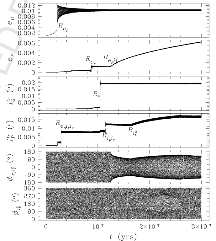
Fig. 5. The PG\ 2:1 passage with an isolated eccentricity-type resonance capture; we show eccentricities, free inclinations and the two relevant resonant argument. As in Fig. 3, the initial e_G \neq 0 is forced by the strong nearby R_{eG} resonance. After trapping into the R_{ePiT} resonance at t \approx 1.2 \times 10^7 yrs, Proteus is captured into the second-order resonance ( R_{iP} ) at t \approx 1.6 \times 10^7 yrs which affects its inclination. The second capture is enabled by extremely slow changes to \dot{\varpi}_P and \dot{\Omega}_P induced by the first resonance. In this simulation, \bar{\rho} = 0.8\text{ g/cm}^3 and Q_N = 22,000 .
