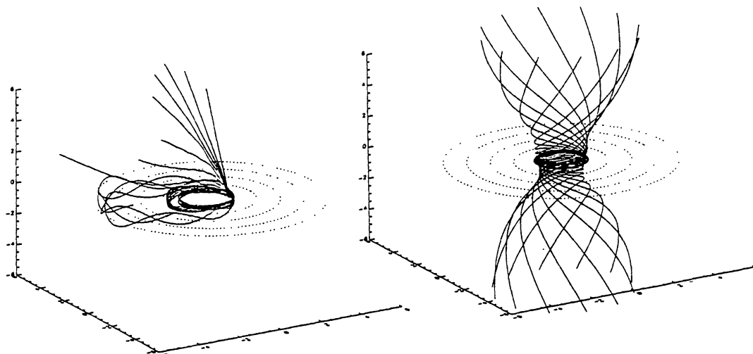
Fig. 1: Orbits in a focusing field (Inner solid oval is Earth's orbit)
