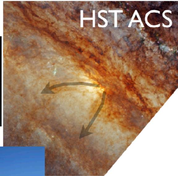
NGC 253: optical
