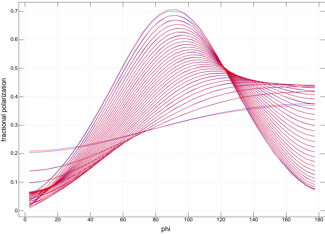
Analytic (blue) vs Monte Carlo (red) -- albedo=0.95, mu_in=0.5
