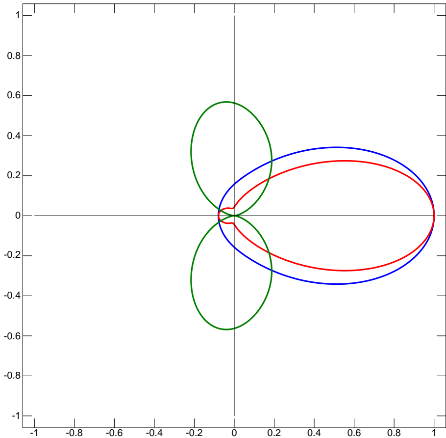
Polar Plot of Scattering Phase Function
