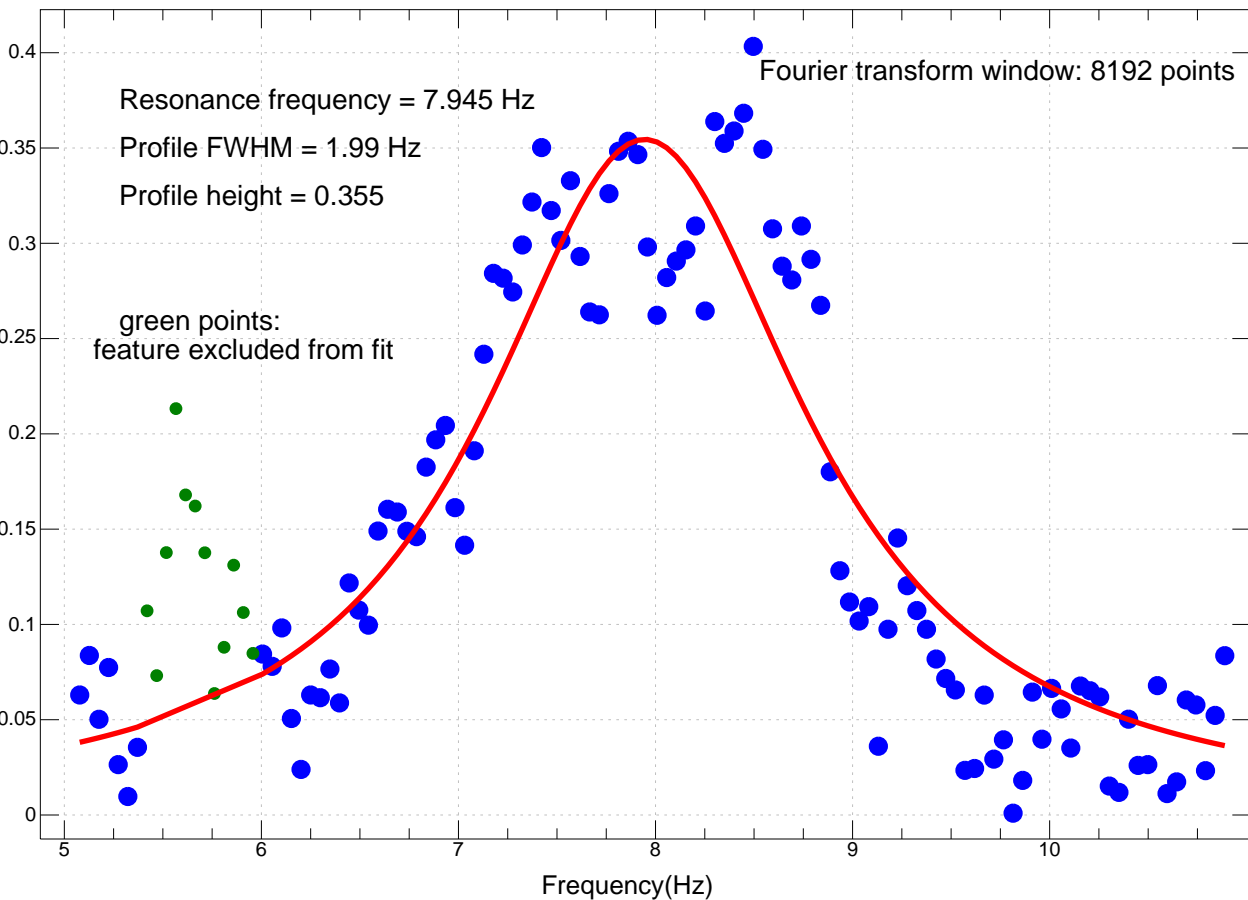
Lorentzian fit to first Schumann resonance. Data from Rocky Point Park, MD - 5 Dec 2021
