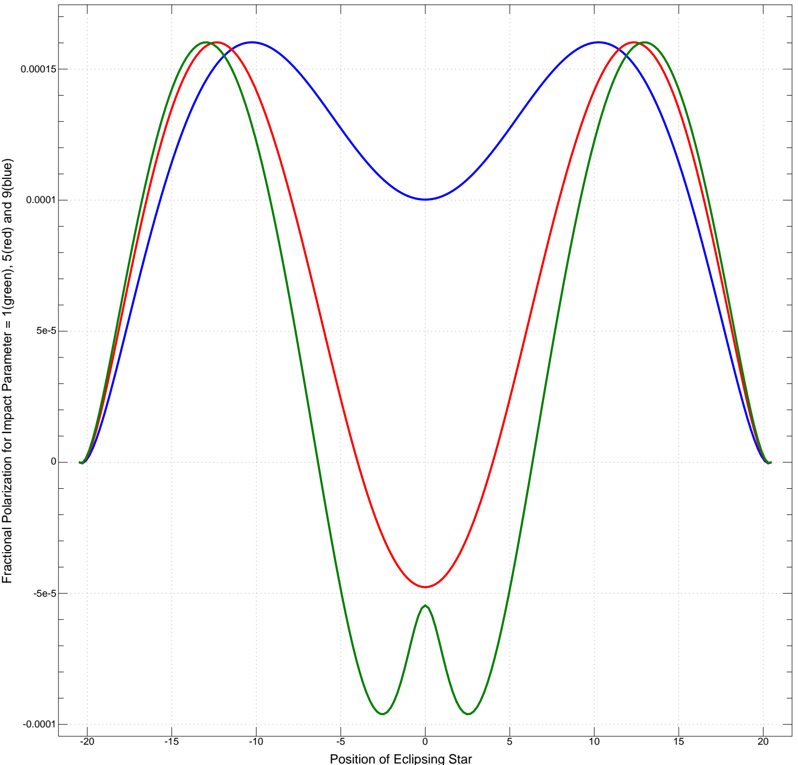
Polarization Curves for Eclipse of Two 10 Solar Radius O-stars
