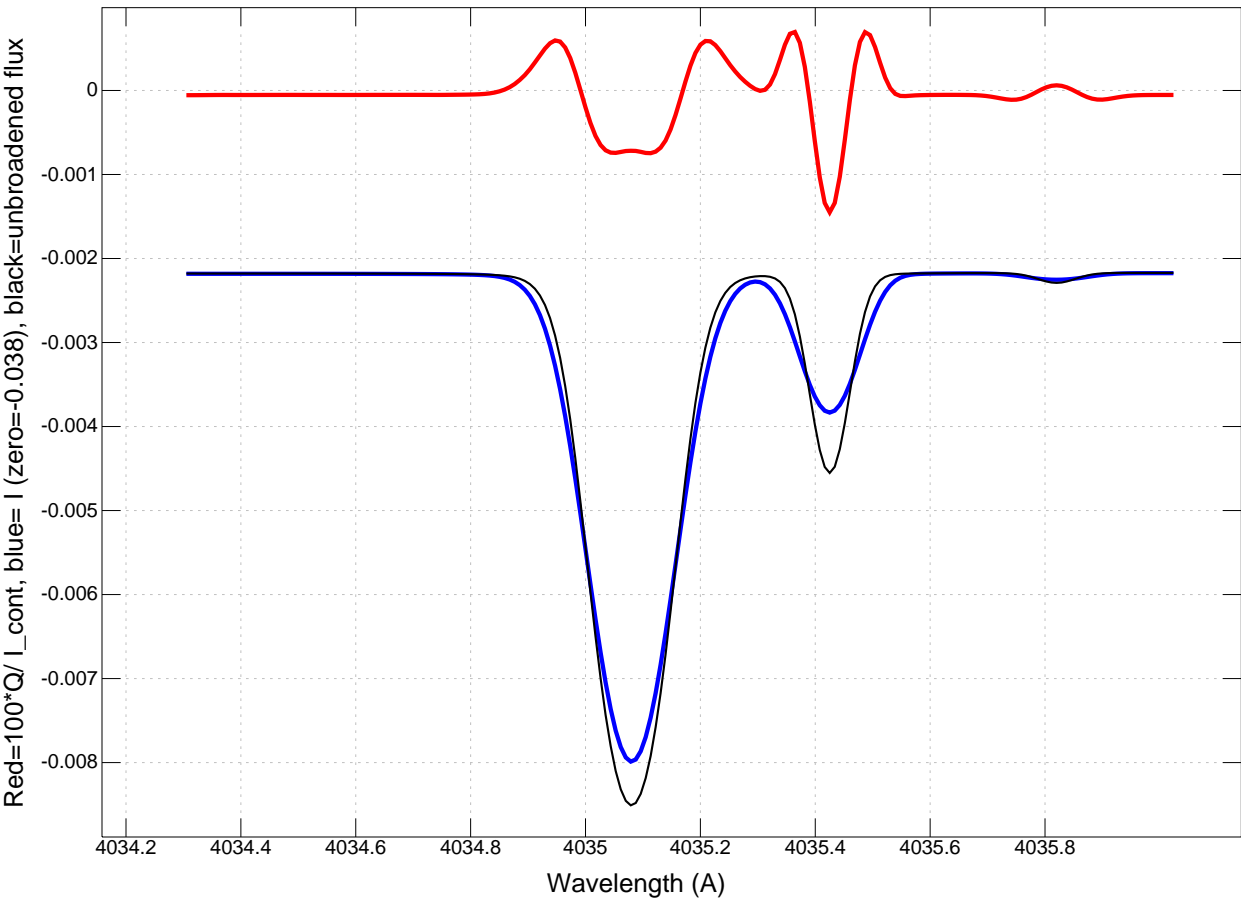
Stokes I&Q across lines of rotating star: T=30,000K, I_g=4.0 -- Rot vel = 5 km/s
