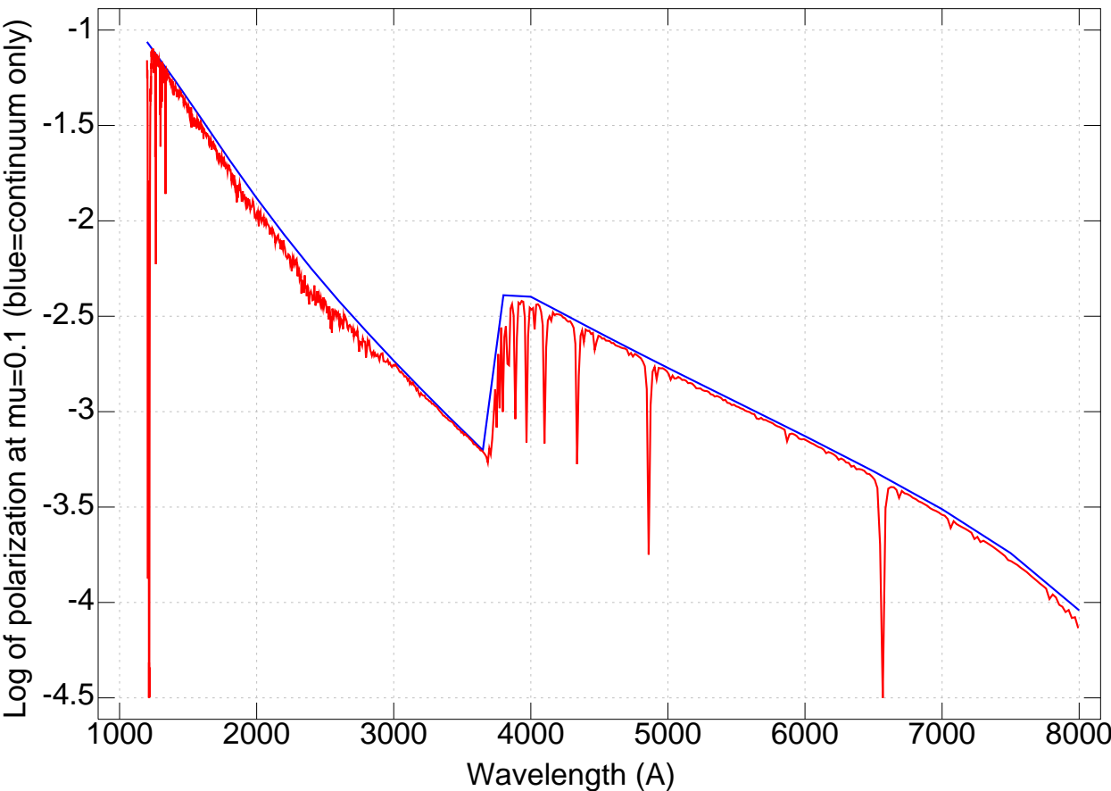
Polarization with/without line blanketing for T=15,000, log g=4.0 TLUSTY model
