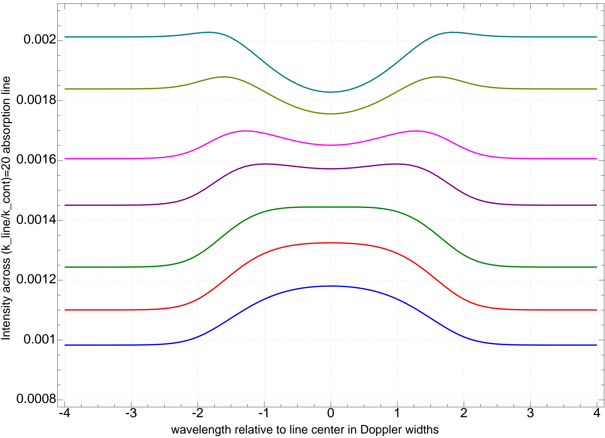
T=30,000K, log g=3, 5000Å. Profiles at \mu=0.7, 0.5, 0.3, 0.2, 0.1, 0.05, 0.02
