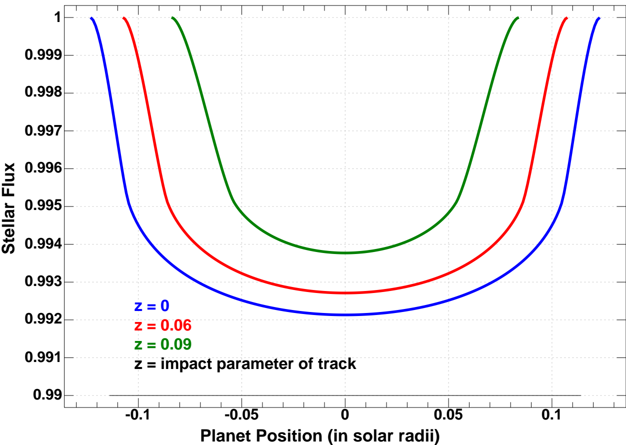
Transit of Earth-size planet across TRAPPIST-1 ( T = 2550 K, \log g = 5.0 ) @ 4600Å
