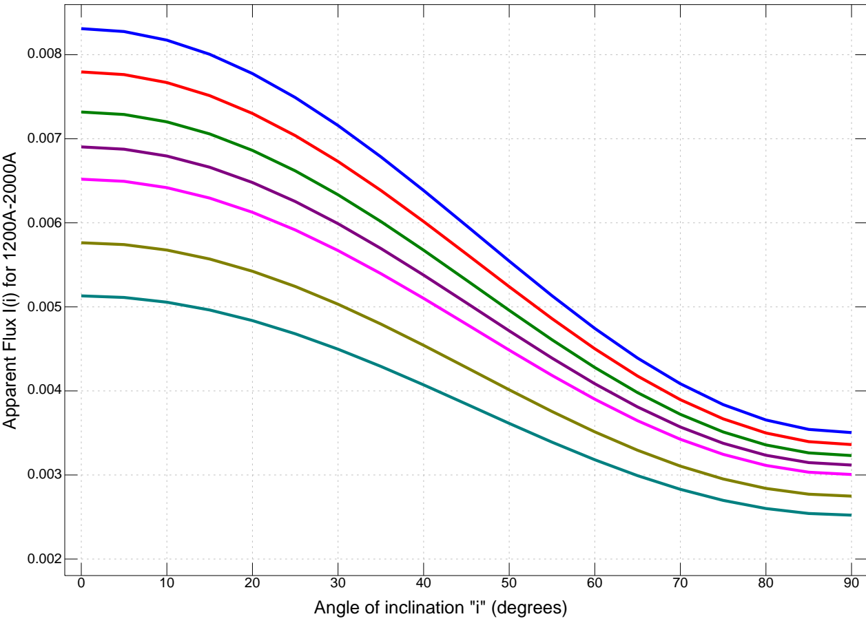
B1 V star at w=0.95 , \lambda=1200, 1300, 1400, 1500, 1600, 1800, 2000\text{\AA}
