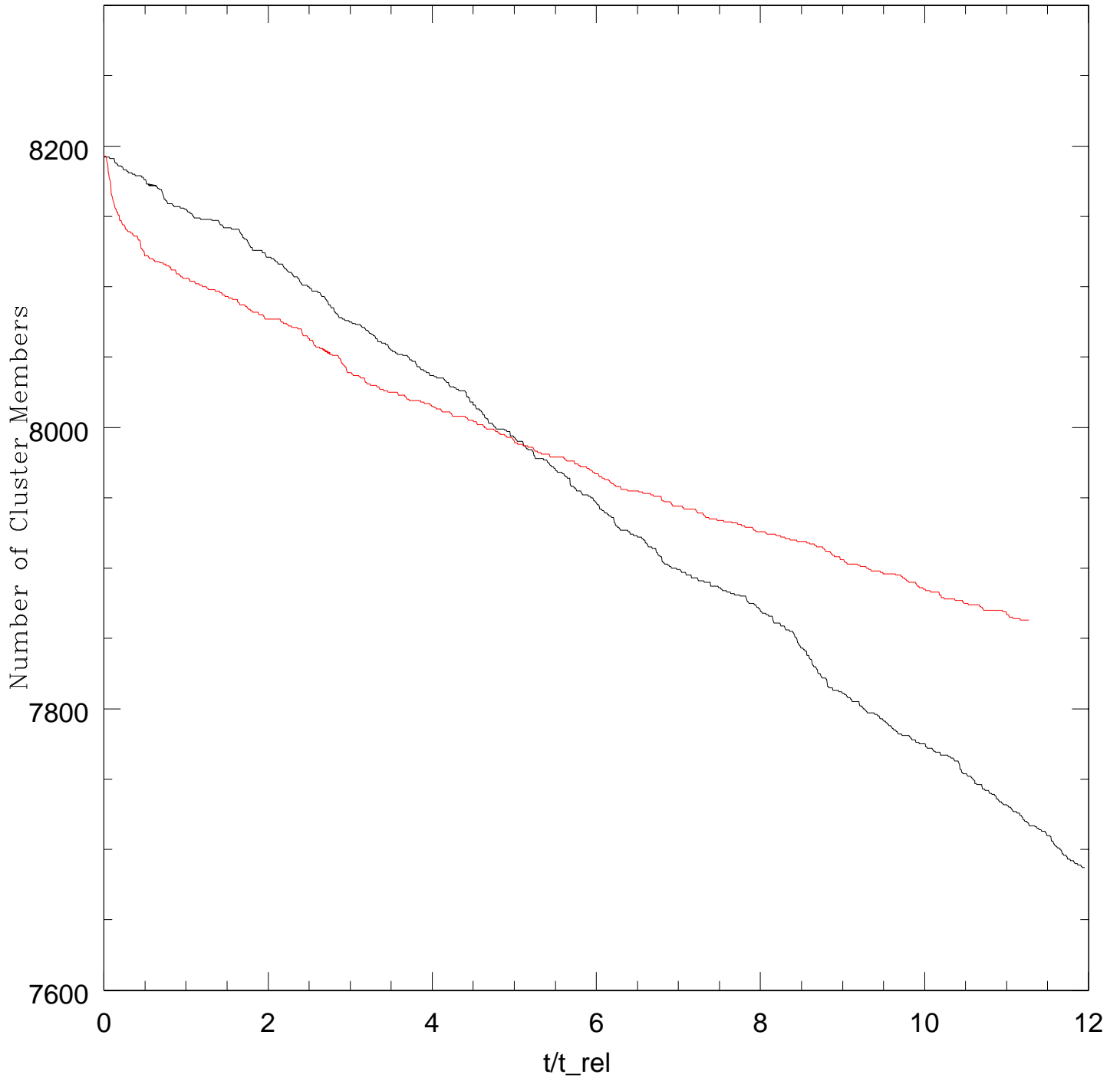
Evolution of Number of Stars in Cluster
