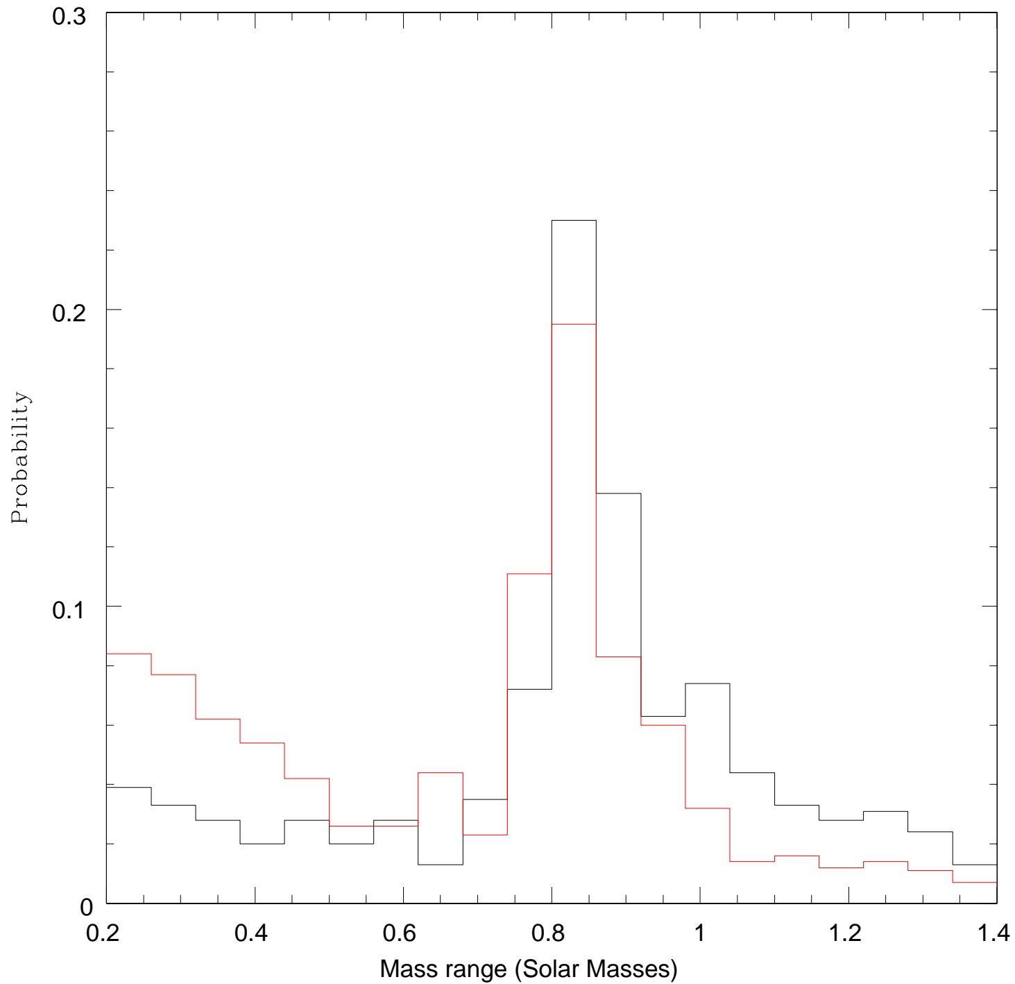
Comparison of Final Probability Distributions of Inner 10% with and without a BH
