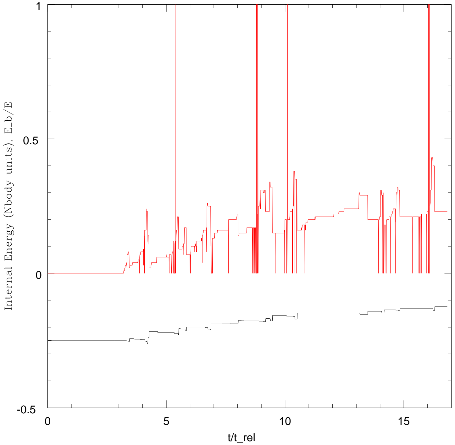
Evolution of Cluster Internal Energy and E_b/E
