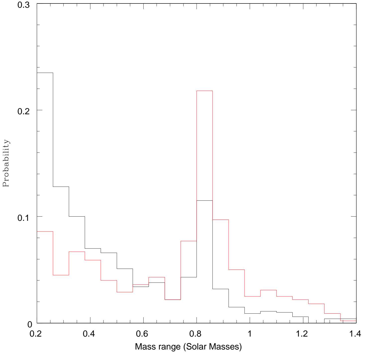
Probability Distribution of Masses in the Inner 10%
