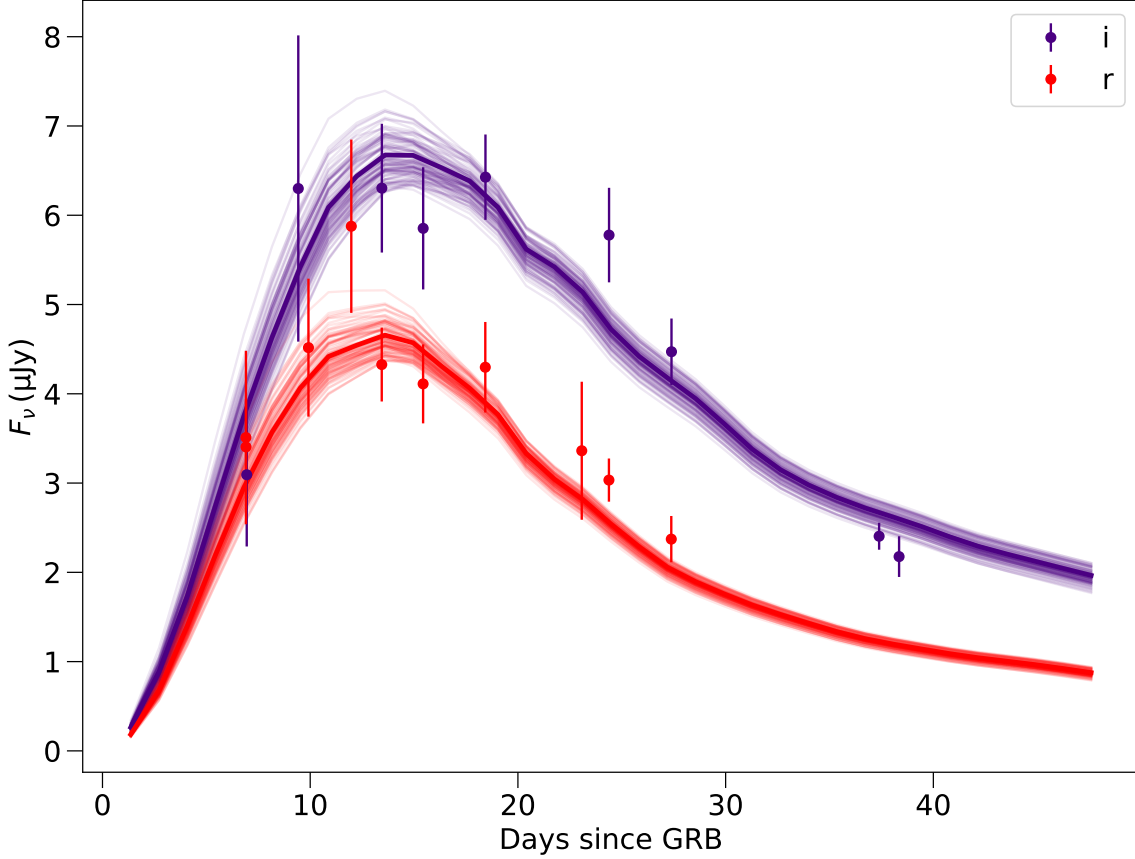
Figure 5. The afterglow-subtracted SN flux LC of SN 2023pel, corrected for Galactic extinction. In addition, we plot the best-fit r and i -band flux LCs in the observer frame obtained from the best-fit bolometric LC constructed from the A82 radioactive heating SN model, assuming the color and spectral evolution of SN 2023pel is identical to that of SN 2002ap. We derive the best-fit values M_{\text{Ni}} = 0.38 \pm 0.01 M_{\odot} , \tau_{\text{m}} = 7.64^{+0.34}_{-0.33} days. 100 random a posteriori possible models from the MCMC fitting samples are also plotted with the best fits shown in bold.
