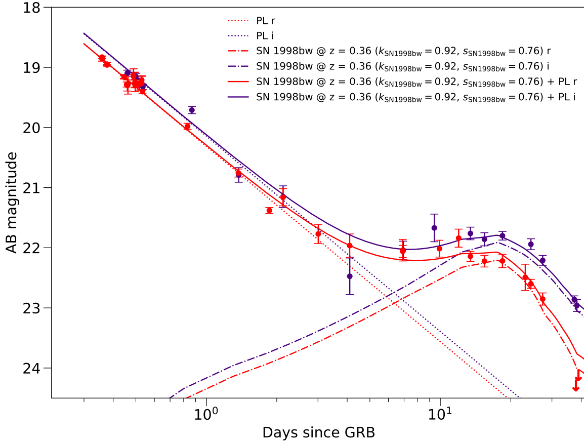
Figure 3. Observed r and i band photometry of GRB 230812B from the optical instruments listed in §2. The photometry values are reported in Table 1, and all times are in the observer frame. We also show the best-fit power law decay to the optical data derived in §3.1, corresponding to a power-law decay index of \alpha = 1.31 . The LCs for a SN 1998bw-like source in r and i bands, redshifted to z = 0.36 , reddened according to the line-of-sight Galactic extinction of GRB 230812B, with a flux-stretching factor of k = 0.92 and time-stretching factor of s = 0.76 (derived in §3.2) applied, are also shown.
