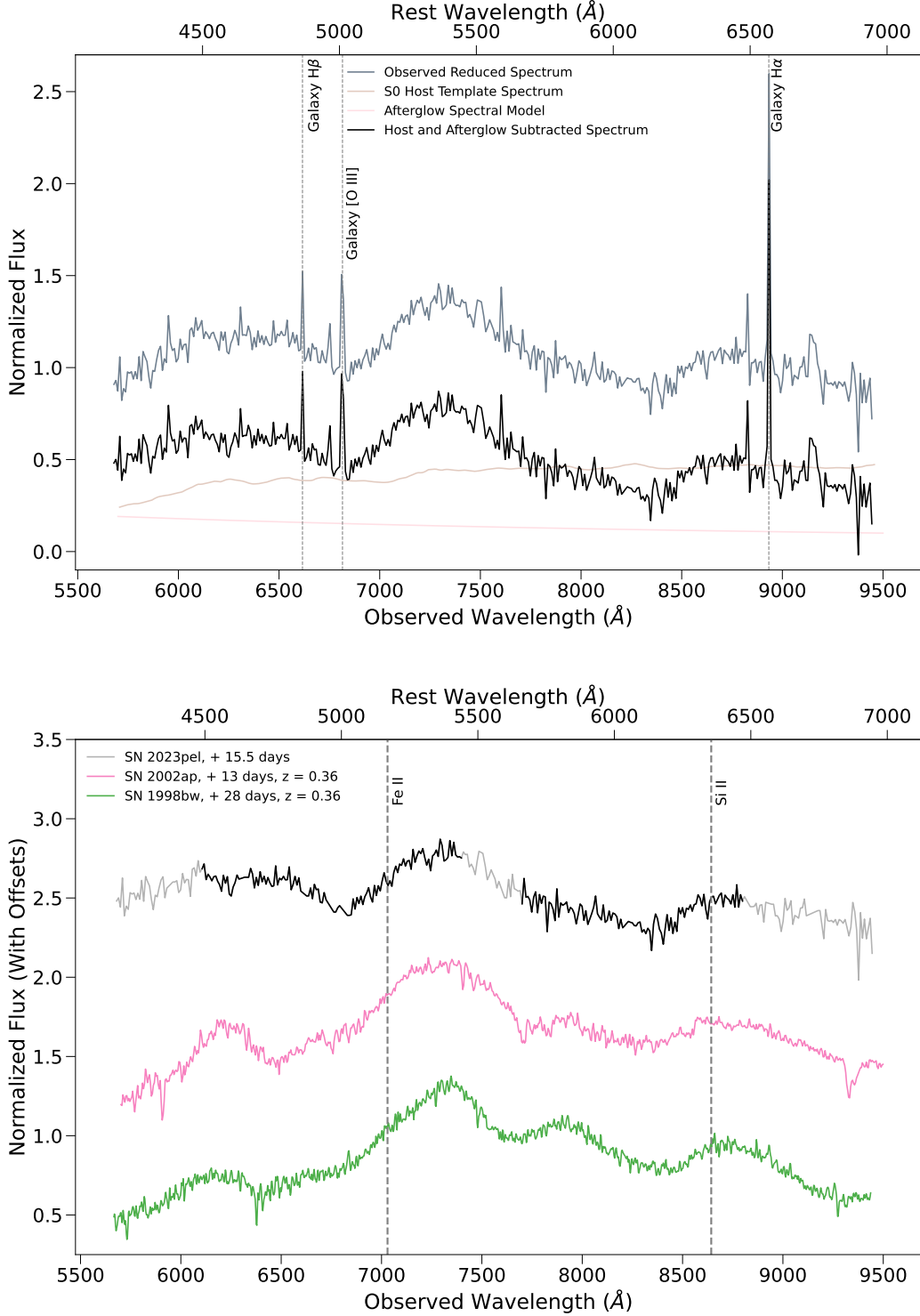
Figure 6. Top panel: DEIMOS spectrum obtained of GRB 230812B/SN 2023pel, 15.5 days after the observed peak in r band. We show the original reduced spectrum, the best-fit S0 host galaxy template spectrum from NGSF with its flux scaled to the time of the spectrum, the afterglow spectral model with its flux scaled to the time of the spectrum assuming F_\nu \propto \nu^{-\beta_0} (where \beta_0 = 0.74 is the optical spectral index), and the final, host and afterglow-subtracted spectrum of SN 2023pel, smoothed and normalized for display purposes. The spectrum shows the strong H \beta , H \alpha , and [O III] galaxy emission lines at z = 0.36 . Bottom panel: We show the spectrum of SN 2023pel, after manually removing narrow galaxy emission lines. We also show the observed spectrum of SN 2002ap, 13 days after peak, and redshifted to z = 0.36 , and of SN 1998bw, 28 days after peak, also redshifted to z = 0.36 . All three spectra show broad Fe II and Si II features, characteristic of Type Ic-BL SNe, and we label the lines as well as show the broadened features in bold for SN 2023pel.
