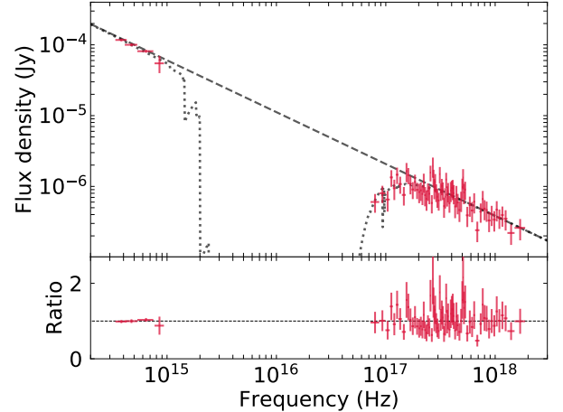
Figure 2. Broadband modeling of the GRB afterglow from optical (ZTF and SEDM; ugri ) to X-ray ( Swift ) wavelengths at a midtime of T_0 + 8.8 hours. The model is a simple absorbed power-law shown by the gray dotted line and the unabsorbed model is shown as the gray dashed line, both corrected for Galactic extinction. The bottom panel shows the ratio between the data and the absorbed power-law model with the black dashed line showing a ratio of unity.
