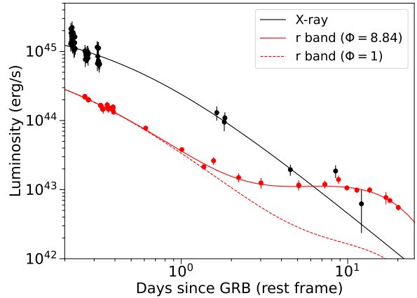
Figure 4. The magnetar model from Cano et al. (2016) fit to both the Swift XRT X-ray LC and r -band LC of GRB 230812B/SN 2023pel independently. The properties of the magnetar derived are not consistent when comparing the X-ray and optical analysis, where we find that B_0 = 3.37^{+0.91}_{-0.63} \times 10^{15} \text{ G} and P_0 = 14.44^{+2.29}_{-1.93} \text{ ms} from the X-ray fitting, and B_0 = 1.07^{+0.13}_{-0.12} \times 10^{16} \text{ G} and P_0 = 32.41^{+2.67}_{-2.48} \text{ ms} from the optical fitting. We find that an additional flux-stretching factor of \Phi = 8.84^{+0.62}_{-0.63} is necessary to fit for the SN bump in the r -band LC, and we show the r -band LC with and without the inclusion of this stretching factor in the plot. These findings all show that the magnetar model is not viable to describe the LC of GRB 230812B/SN 2023pel, and that an additional source of power is necessary to describe the observed flux.
