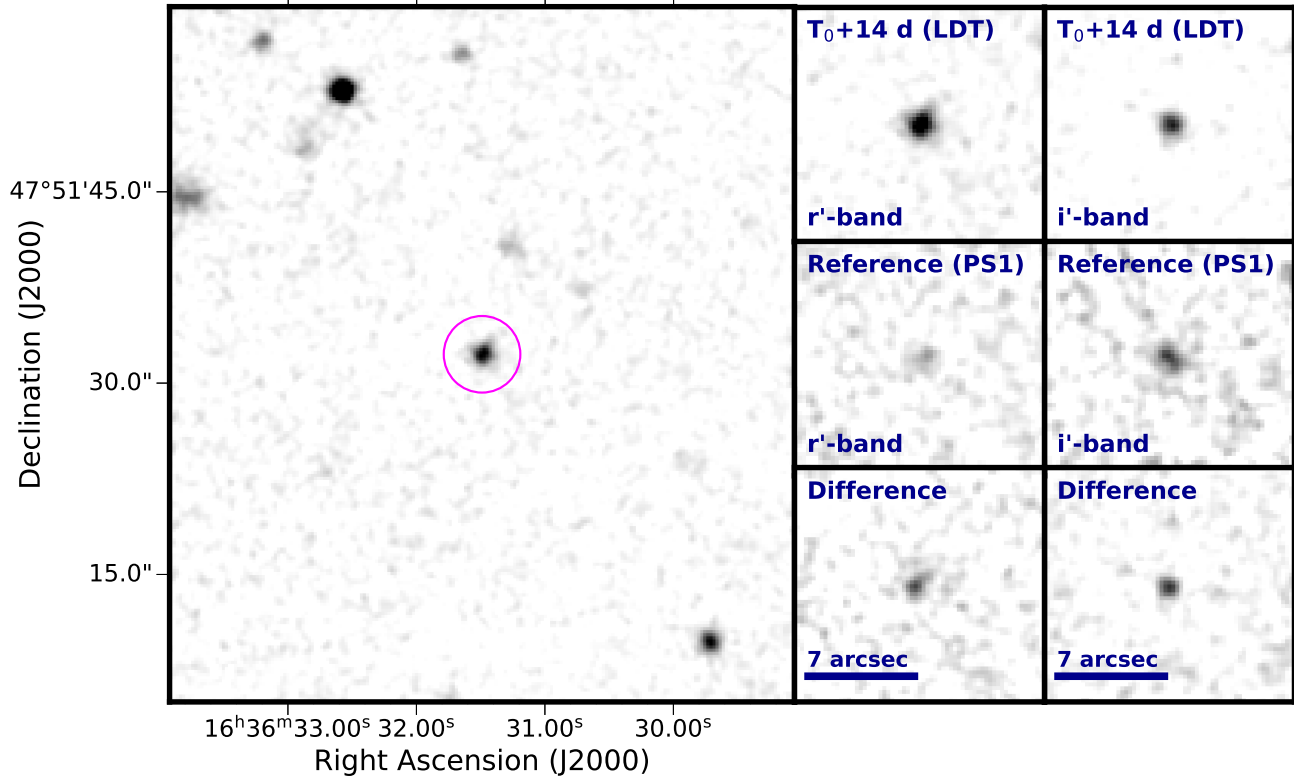
Figure 1. LDT images of the optical afterglow of GRB 230812B/SN 2023pel. The left, large panel shows the wider field of view of GRB 230812B, in r band 14 days after T_0 . The right panels show the observations taken of the GRB that include the host galaxy contribution, the reference images from PS1 used for image subtraction, and the resulting subtracted images used for photometry, in both r and i bands. The images have been smoothed for display purposes.
