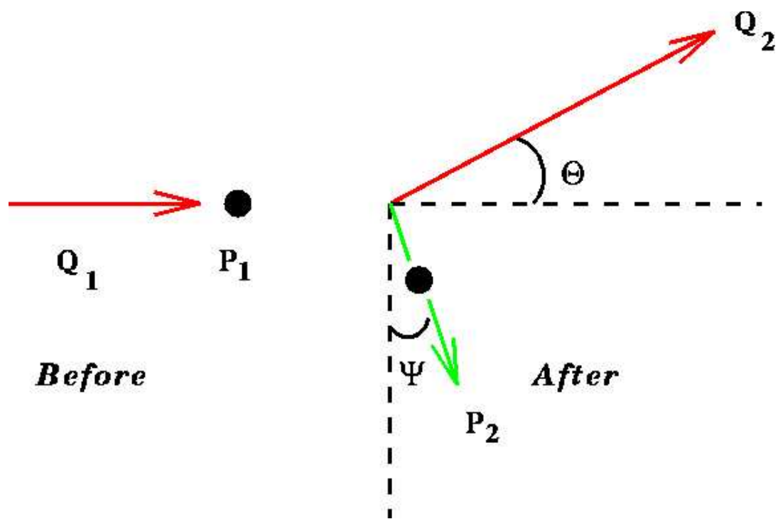
Fig. 1.— Diagram of Compton scattering. From http://www.mth.uct.ac.za/omei/gr/chap2/img137.gif
