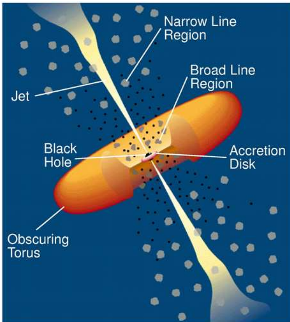
Fig. 1.— Schematic of an active galactic nucleus. The central engine is the black hole; around it is an accretion disk. Jets, which originate from outside the black hole, are along the black hole spin axis and perpendicular to the disk. Figure from http://perry.sonoma.edu/gamma2001/wednesday/badran-horan/images/agn_up_model.png
