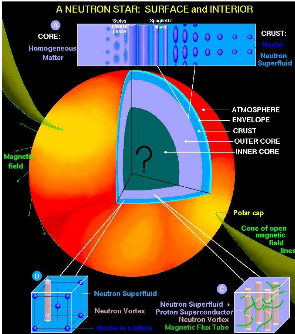
Fig. 1.— Figure showing many aspects of neutron stars that are discussed in this lecture. Originally due to Dany Page.
