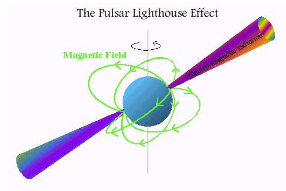
Fig. 1.— The lighthouse model of pulsars. A beam of radio waves, tied to the surface of the star, sweeps past us as the star rotates. From http://www.astro.cornell.edu/academics/courses/astro201/images/pulsar.gif
