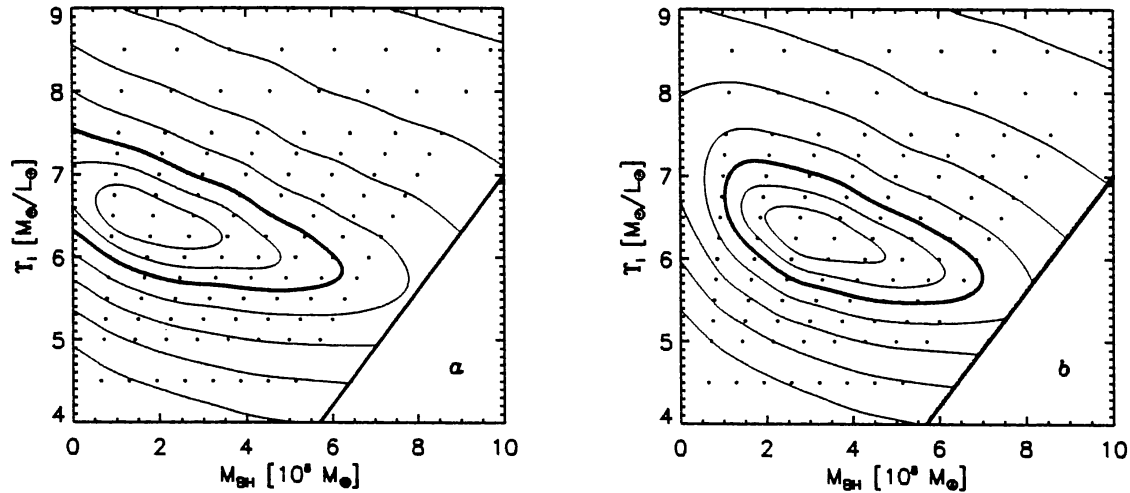
Figure 2. Contour plots of \chi^2 which measures the goodness-of-fit to the data as function of BH mass and I -band M/L -ratio. The first three contours define the formal 68.3, 95.4 and 99.73 confidence levels. Solid dots indicate actual model calculations. The \chi^2 surface of panel a result from only including the WHT data. Including the HST data as well, results in the \chi^2 surface of panel b . Clearly, the higher spatial resolution HST data allows us to rule out models without BH to a confidence level better than 99.73 per cent.
