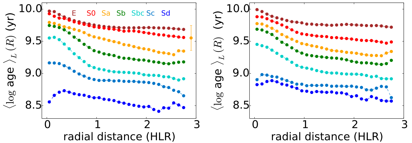
Fig. 9. Radial profiles of \langle \log age \rangle_L as a function of Hubble type (left) and in seven bins of galaxy stellar mass (right). These bins are \log M_\star (M_\odot) = 9.1-9.6, 9.6-10.1, 10.1-10.6, 10.6-10.9, 10.9-11.2, 11.2-11.5, 11.5-11.8 . Symbols and colors are as in Fig. 6. These results are obtained with base GMe .
