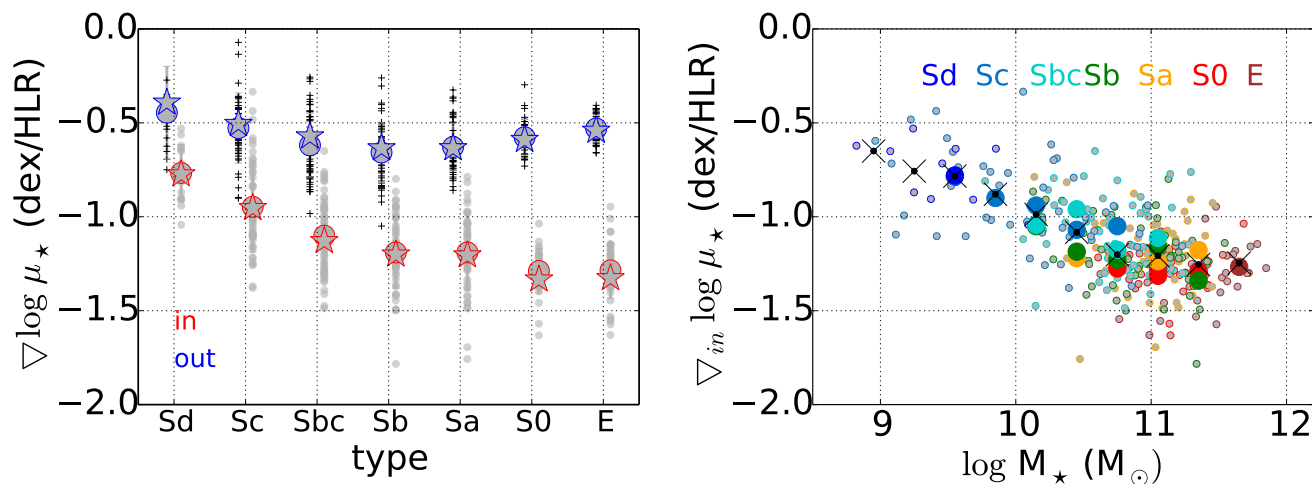
Fig. 7. (left) Correlation between the inner (grey-red) and outer (grey-blue) gradient of \log \mu_* and the morphological type. The results are shown for the GMe (stars) and CBe (circles) SSP models. The inner gradient is calculated between the galaxy nucleus and 1 HLR, and the outer gradient between 1 HLR and 2 HLR. (right) Correlation between the inner gradient of \log \mu_* and the galaxy stellar mass. Small dots represent the results for each galaxy, and black crosses show the average for each 0.3 dex mass bin. Large circles represent the averaged inner gradient in mass intervals of 0.3 dex for each color-coded morphological type. Black crosses show the average correlation between the inner gradient of \log \mu_* and galaxy mass independently of the morphological type.
