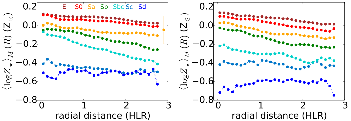
Fig. 12. Radial profiles of \langle \log Z_{\star} \rangle_M as a function of Hubble type (left) and of galaxy stellar mass (right). Mass bins are \log M_{\star} (M_{\odot}) = 9.1-9.6, 9.6-10.1, 10.1-10.6, 10.6-10.9, 10.9-11.2, 11.2-11.5, 11.5-11.8 . Symbols and colors are as Fig. 6. These results are obtained with base GMe .
