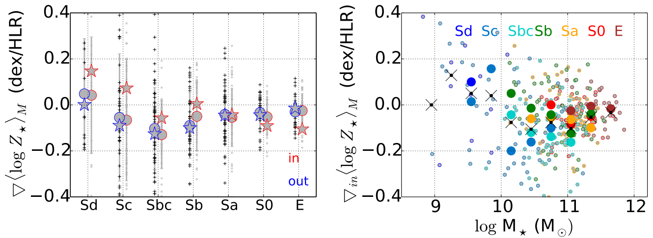
Fig. 13. Left: As Fig. 7 but for \langle \log Z_{\star} \rangle_M . Right: The inner gradient as a function of the galaxy stellar mass. Symbols and colors are as in Fig. 7.
