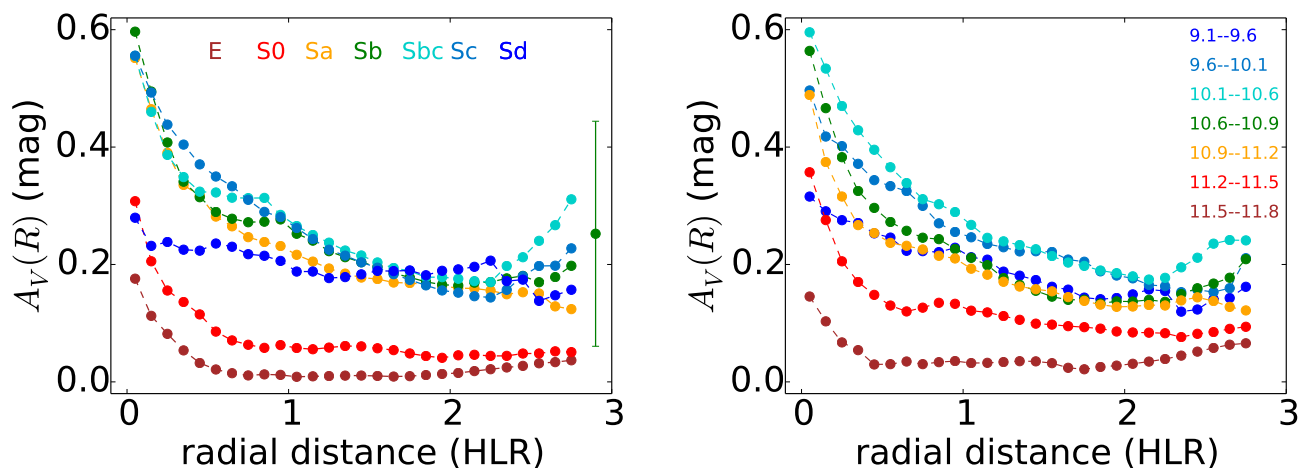
Fig. 15. Radial profiles of A_V as a function of Hubble type (left), and in seven bins of galaxy stellar mass (right). These bins are \log M_*(M_\odot) = 9.1-9.6, 9.6-10.1, 10.1-10.6, 10.6-10.9, 10.9-11.2, 11.2-11.5, 11.5-11.8 . Symbols and colors are as Fig. 6. These results are obtained with base GMe .
