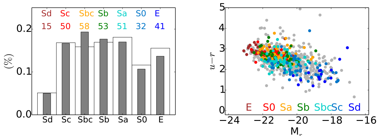
Fig. 1. Left: Comparison of the distribution of Hubble types in the CALIFA mother sample (empty bars) and the galaxies analyzed here (filled bars). The number of galaxies in our sample are labeled in colors. The histograms are normalized to form a probability density, i.e., each bar scales with the ratio of the number of galaxies in each bin and the total number of galaxies, such that the two distributions are directly comparable. Right: Color-magnitude diagram. Mother sample galaxies are plotted in grey, while the 300 galaxies analyzed in this work are marked as colored points.
