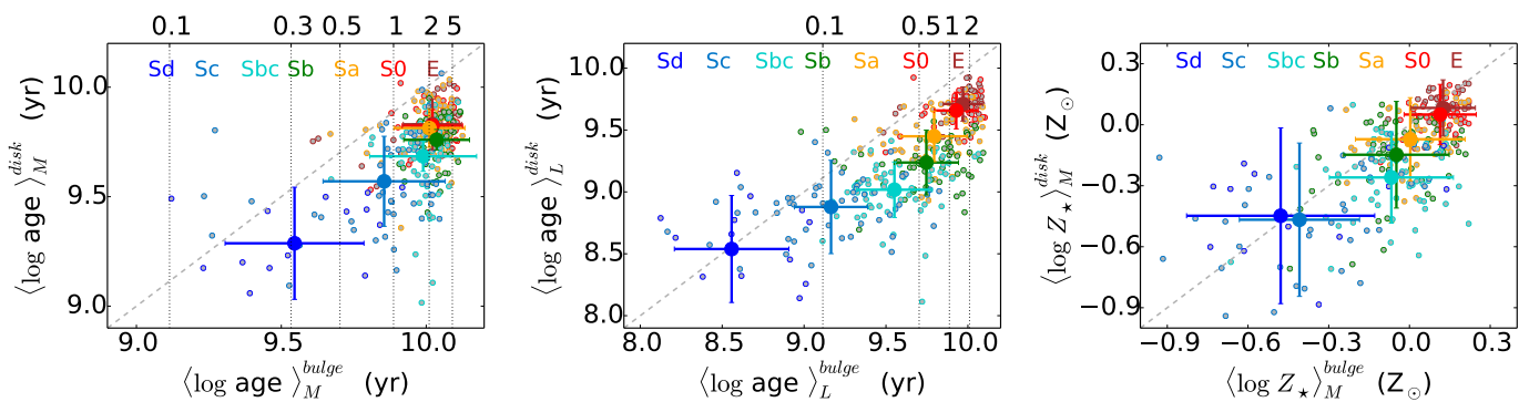
Fig. 18. Left: Mass-weighted age at the galaxy center ( \langle \log age \rangle_M^{bulge} ) and at 1.5 HLR ( \langle \log age \rangle_M^{disk} ) for the different Hubble types. Small dots are the individual radial points, while big colored dots represent mean values for each Hubble type, with the error bars indicating the dispersion in the mean. Middle: As in the left panel but for the light-weighted age ( \langle \log age \rangle_L ). Right: As in the left panel for \langle \log Z_\star \rangle_M . The top horizontal axes in the left and middle panels show the redshift scale. The diagonal line in the three panels is the bisector.
