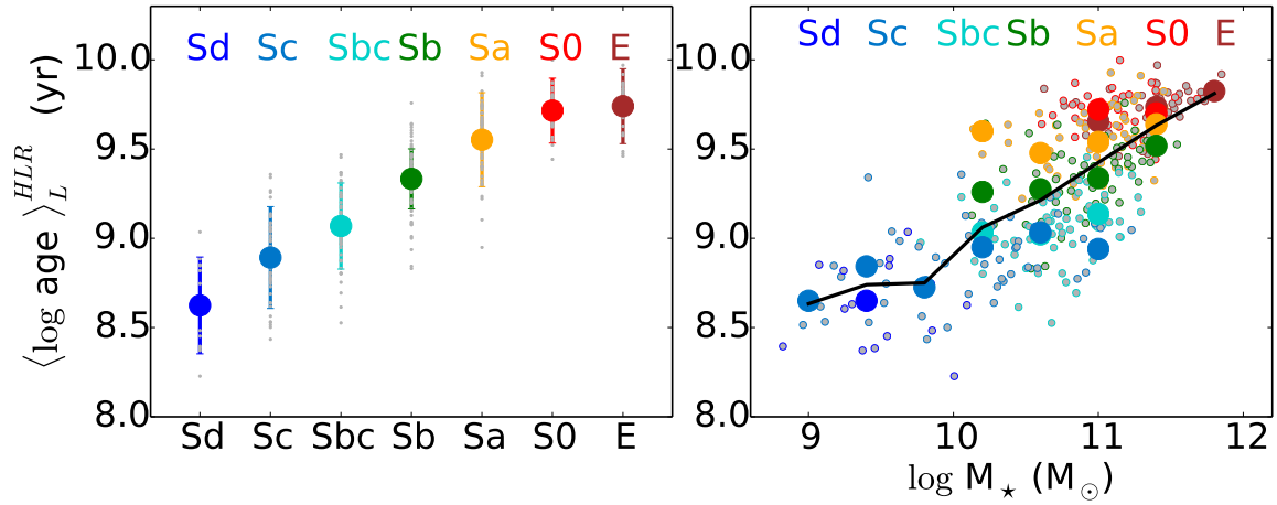
Fig. 8. \langle \log age \rangle_L measured at 1 HLR as a function of Hubble type (left) or galaxy stellar mass (right). Symbols and colors are as in Fig. 5. The black line is the average \langle \log age \rangle_L in galaxy stellar mass bins of 0.4 dex.
