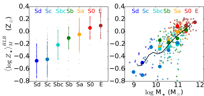
Fig. 11. \langle \log Z_{\star} \rangle_M measured at 1HLR as function of Hubble type (left) and galaxy stellar mass (right). Symbols and colors are as in Fig. 5. The black line is the average \langle \log Z_{\star} \rangle_M obtained in 0.4 dex bins of \log M_{\star} .
