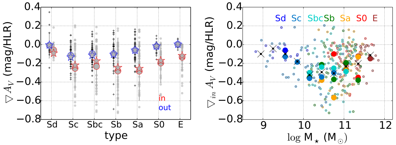
Fig. 16. Left: As Fig. 7 but for A_V . Right: The inner gradient as a function of galaxy stellar mass. Symbols and colors are as in Fig. 7.
