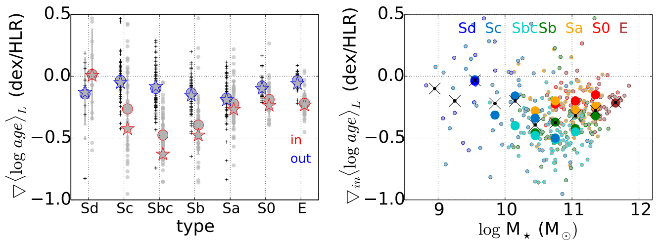
Fig. 10. (left) As Fig. 7 but for \langle \log age \rangle_L . The inner gradient shows a clear dependence with Hubble type, that seems to be stronger than with the galaxy mass. Sb-Sbc-Sc galaxies have larger inner gradients with CBe than with GMe , but both sets of models show a similar dependence with Hubble type. (right) The inner gradient of \langle \log age \rangle_L as a function of galaxy mass. Colors and symbols are as in Fig. 7.
