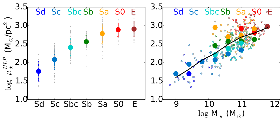
Fig. 5. Left panel: stellar mass surface density measured at 1 HLR as a function of Hubble type. Small dots represent \log \mu_* for each galaxy; the colored circles are the average \log \mu_* for each Hubble type, and the error bars are the dispersion in \log \mu_* for each morphological type. Right panel: \log \mu_* - \log M_* relation. Individual galaxies are represented by their morphological type. The black line is the average \log \mu_* in galaxy stellar mass bins of 0.4 dex. Large colored circles are the average \log \mu_* in each bin of mass for each Hubble type.
