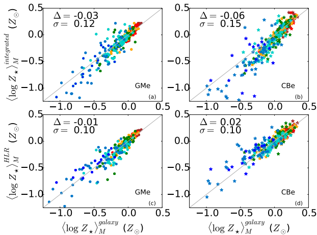
Fig. 4. Upper panels: Comparison of the galaxy-wide average stellar metallicity (weighted in mass) derived from the spatially resolved spectral analysis ( \langle \log Z_{\star} \rangle_M^{galaxy} ) and the integrated metallicity derived from fitting the total (integrated) galaxy spectrum ( \langle \log Z_{\star} \rangle_M^{integrated} ). Lower panel: Comparison of \langle \log Z_{\star} \rangle_M^{galaxy} with the value measured R = 1 HLR ( \langle \log Z_{\star} \rangle_M^{HLR} ). Left and right panels show results obtained with base GMe and CBe SSPs, respectively. All panels include 300 galaxies. The difference between the y-axis and x-axis is labeled in each panel as \Delta , and the dispersion as \sigma .
