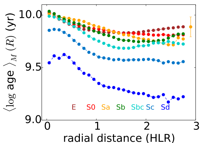
Fig. 19. Radial profiles (in units of HLR) of the mass weighted age, \langle \log age \rangle_M^{bulge} , obtained with GMe base. The results are stacked by morphological type as in Fig. 7.
