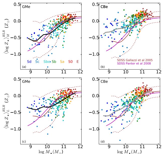
Fig. B.1. The global stellar MZR for 300 CALIFA galaxies is shown as dots, color coded by the morphological type. It is derived using \langle \log Z_\star \rangle_M^{HLR} (upper panels) and \langle \log Z_\star \rangle_L^{HLR} (lower panels), and the total stellar mass, M_\star , obtained with the GMe SSP models (left panels) and CBe (right panels). A mass-binned smooth mean relation is shown as a solid black or grey-black line. The MZR obtained for SDSS galaxies by Gallazzi et al. (2005) and Panter et al. (2008) are plotted as brown and magenta lines, respectively, with dashed brown indicating the 16 and 84 percentiles of Gallazzi et al. (2005).
