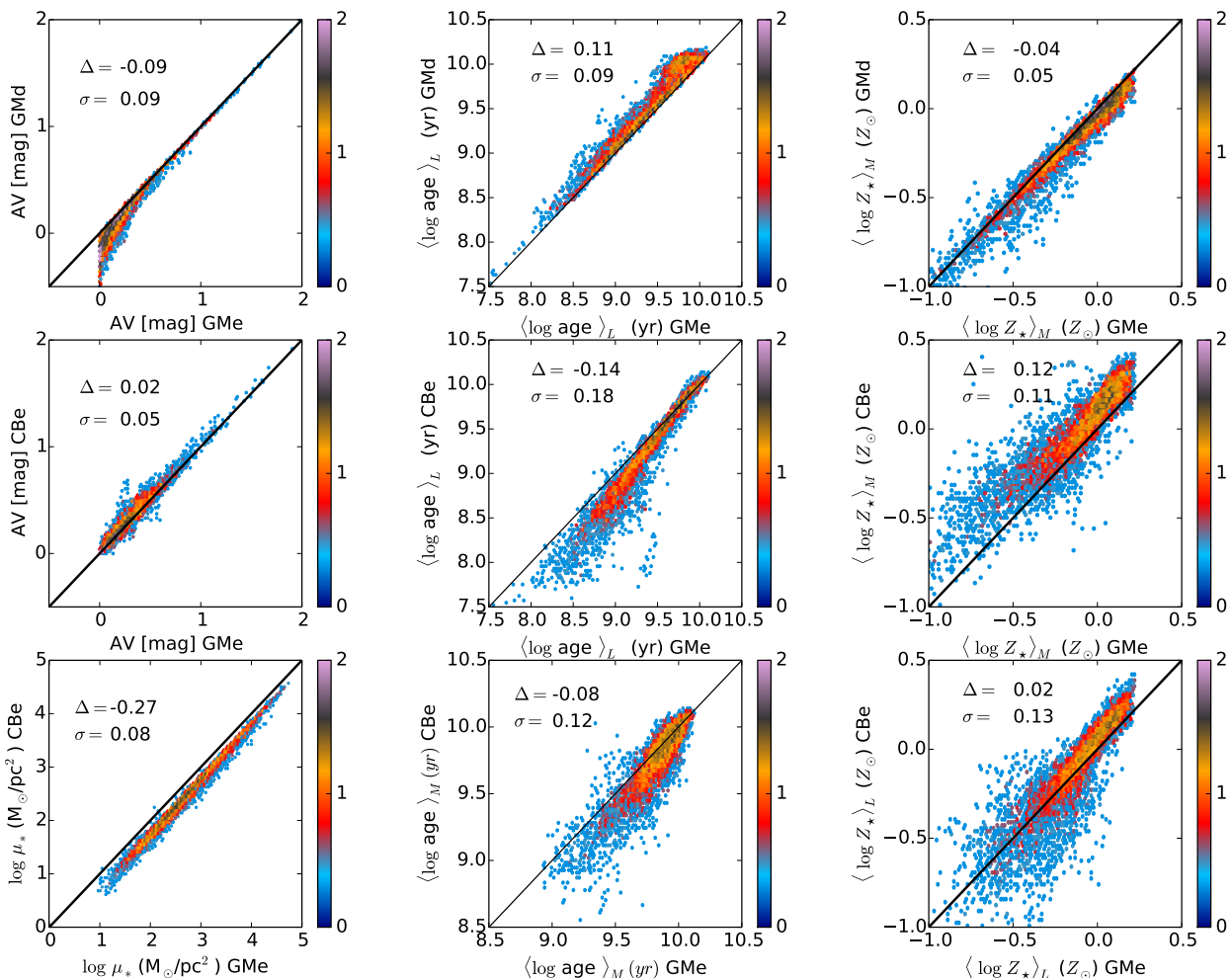
Fig. B.2. Correlation between SP obtained with the GMe (x-axis) and CBe (y-axis bottom and middle panels; and GMe (x-axis) and GMd (y-axis). The average difference between the property in the y-axis and x-axis is labeled in each panel as \Delta , and the dispersion as ( \sigma ).
