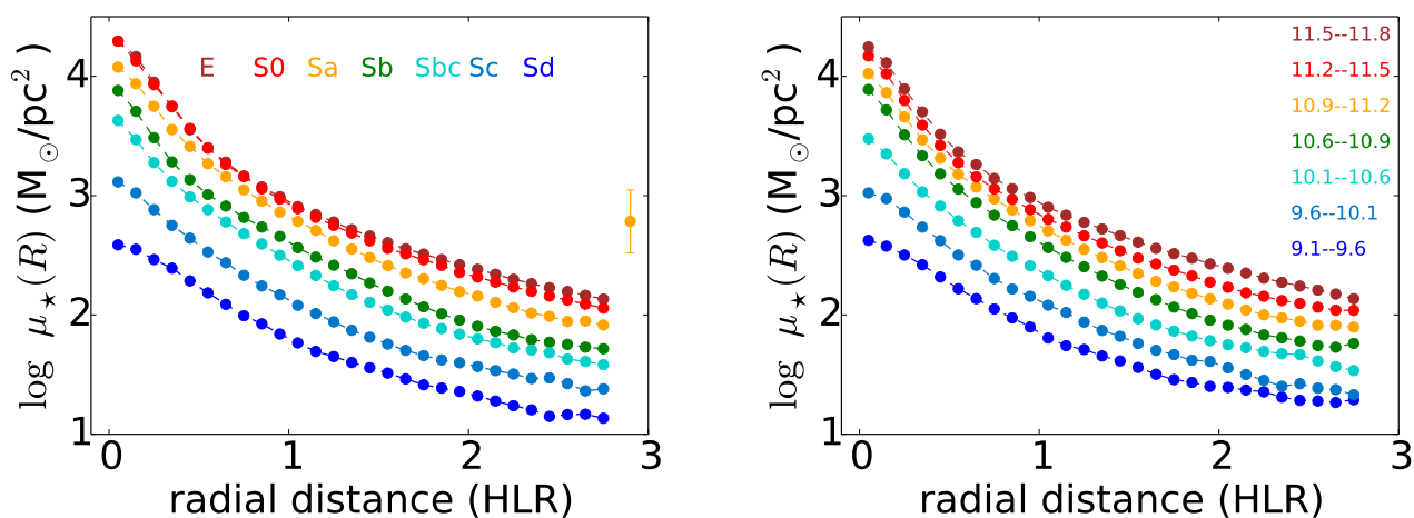
Fig. 6. (left) Radial profiles (in units of HLR) of the stellar mass surface density obtained with base GMe . The results are stacked in seven morphology bins. The error bar in the panel indicate the dispersion at one HLR distance in the galaxies of the Sa bin. It is similar for other Hubble types and radial distances. (right) Radial profiles stacked in seven bins of galaxy stellar mass, \log M_*(M_\odot) : 9.1–9.6, 9.6–10.1, 10.1–10.6, 10.6–10.9, 10.9–11.2, 11.2–11.5, 11.5–11.8.
