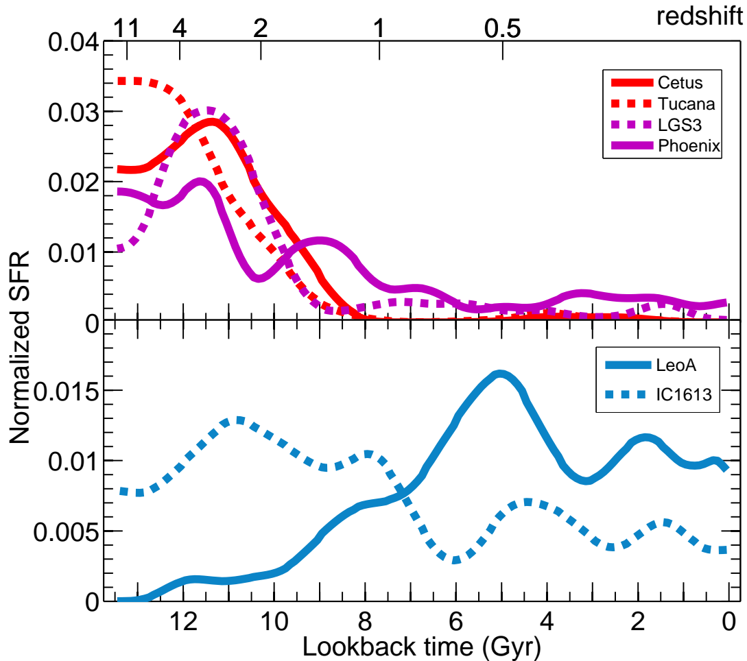
FIG. 1.— Homogeneously derived SFHs for the six LCID galaxies. Upper panel: SFHs for dSph and dT. Lower panel: SFHs for the dIrr.
