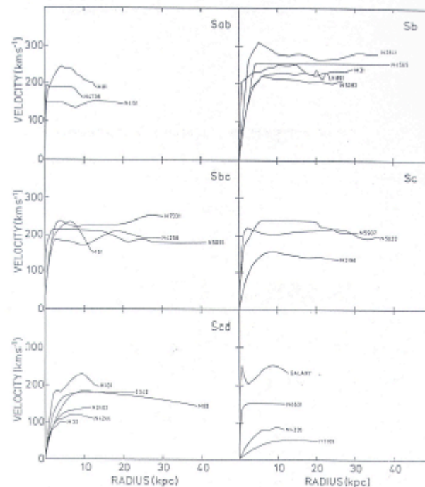
FIGURE 1. Rotation curves of 26 galaxies of various Hubble types.
