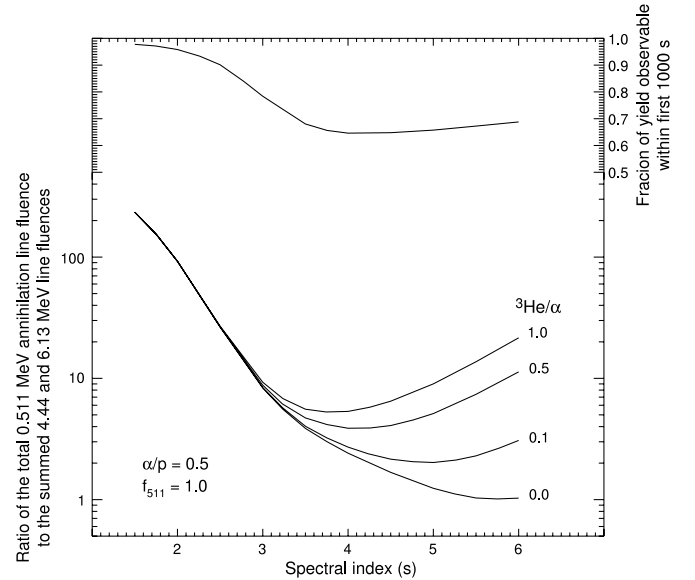
FIG. 8.—Lower curves: Calculated ratio of the total 0.511 MeV positron-annihilation line fluence to the summed fluences of the 4.44 and 6.13 MeV 12 C and 16 O deexcitation lines, as a function of accelerated-particle spectra index s for ^3\text{He}/\alpha = 0, 0.1, 0.5 , and 1.0 . The positron to annihilation-line photon conversion factor f_{511} = 1.0 . Upper curve: Fraction of the total positron annihilation photons observable within the first 1000 s, as a function of the accelerated-particle spectral index.
