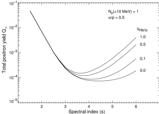
FIG. 7.—Total thick-target positron yield, Q_+ , as a function of the accelerated-particle spectral index for ^3\text{He}/\alpha = 0, 0.1, 0.5 , and 1.0 .
