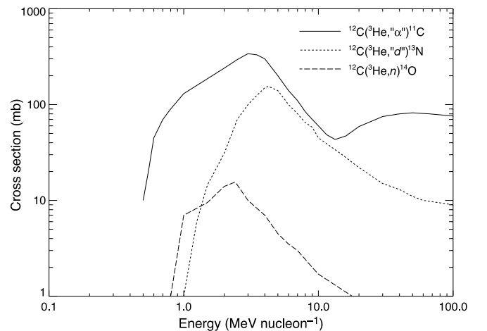
FIG. 1.—Radioactive positron-emitter production cross sections for ^3\text{He} reactions on ^{12}\text{C} .
