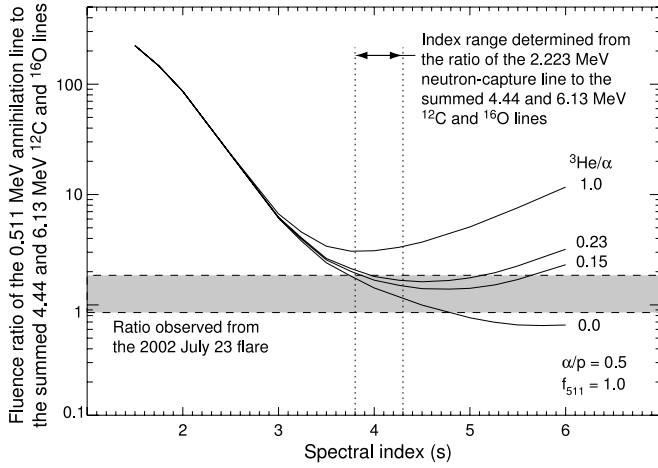
FIG. 9.—Calculated ratio of the 0.511 MeV positron-annihilation line fluence to the summed fluences of the 4.44 and 6.13 MeV ^{12}\text{C} and ^{16}\text{O} de-excitation lines as a function of the accelerated-particle spectral index s for ^3\text{He}/\alpha = 0, 0.15, 0.23 , and 1.0 . The assumed positron to annihilation-line photon conversion factor f_{511} is 1.0 , and all curves have been reduced to account for the fraction of the total annihilation-line fluence observable during the 23 July flare observation interval. The ^3\text{He}/\alpha values of 0.15 and 0.23 are the 90% and 99% confidence upper limits, respectively, determined from the measured ratio of the 0.937 MeV ^{18}\text{F} line fluence upper limit and the \sim 0.45 MeV \alpha - \alpha complex fluence. The horizontal band indicates the ratio ( \pm 1\sigma ) observed by RHESSI from the 2002 July 23 flare. The vertical dotted lines indicate the allowed range ( \pm 1\sigma ) of spectral index derived from the observed fluence ratio of the 2.223 MeV neutron-capture line to the summed 4.44 and 6.13 MeV ^{12}\text{C} and ^{16}\text{O} de-excitation lines.
