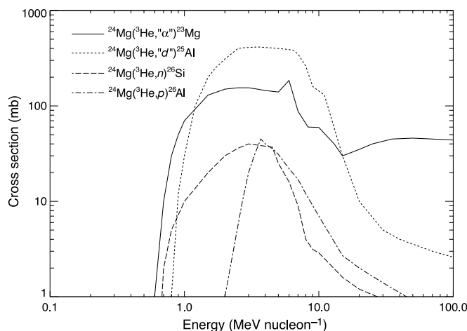
FIG. 4.—Radioactive positron-emitter production cross sections for ^3\text{He} reactions on ^{24}\text{Mg} . These cross sections are also used as the cross sections for the corresponding n , p , d , and \alpha reactions of ^{20}\text{Ne} .
