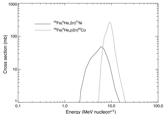
FIG. 6.—Radioactive positron-emitter production cross sections for ^3\text{He} reactions on ^{56}\text{Fe} .
