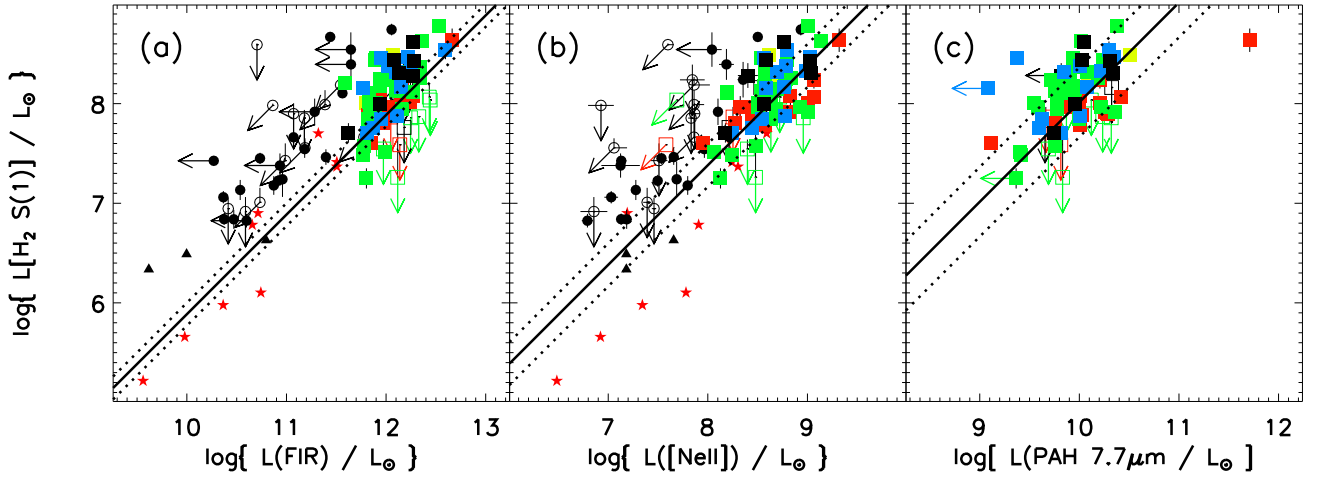
Fig. 29.— Luminosity of \text{H}_2 S(1) 17.04 \mu\text{m} vs. various star formation indicators: (a) FIR luminosity, (b) luminosity of [\text{Ne II}] 12.8 \mu\text{m} , and (c) luminosity of PAH 7.7 \mu\text{m} . The meaning of the square and circle (other) symbols is the same as in Figure 4 (12). The solid and dotted lines show the mean and standard deviation of L[\text{H}_2 \text{ S}(1)]/L(X) (where X = \text{FIR} , etc.) for HII ULIRGs. A positive correlation is seen between these quantities for both ULIRGs and PG QSOs. However, Seyfert ULIRGs and especially PG QSOs have larger \text{H}_2 -to-FIR, \text{H}_2 -to- [\text{Ne II}] , and \text{H}_2 -to-PAH ratios than HII ULIRGs, suggesting that \text{H}_2 emission is influenced by the presence of the AGN in these objects. The LINERs also have significantly larger ratios and dispersions in panels (b) and (c).
