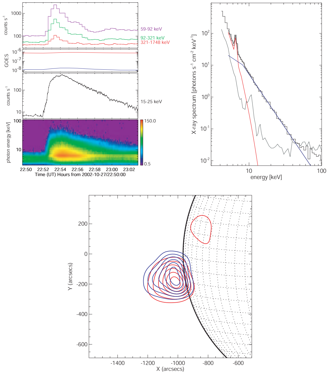
Fig. 7 The 27 October 2002 event (Krucker et al 2007b). This was seen on-disk from Mars by Mars Odyssey , but for Earth-orbiting spacecraft the flare site was occulted by at least 200'' ( 0.2 R_{\odot} ). Top left : the panels show (1) X-ray and \gamma -ray time profiles as seen from Mars (the entire flare), (2) the GOES soft X-ray flux (Earth), (3) RHESSI 15-25 keV time profile (Earth), (4) RHESSI hard X-ray spectrogram (Earth). Top right , the photon spectrum (black) during the exponential decay (22:56:48 to 22:57:00 UTC) with the thermal fit in red and a broken power law fit in blue ( \gamma = 3.4 \pm 0.1 ). The gray line represents the background emission. Bottom , RHESSI X-ray imaging in a thermal range (3-7 keV, red contours) and a non-thermal range (10-30 keV, blue contours) reveal large sources ( >200'' ) seen just above the limb. The RHESSI Clean algorithm was used to reconstruct these images, and the contour levels shown are at 15, 30, 45, 60, 75, and 90 % of the maximum. The thermal emission on disk around (-800, 200) is from AR10717 and is already present before the flare occurs.
