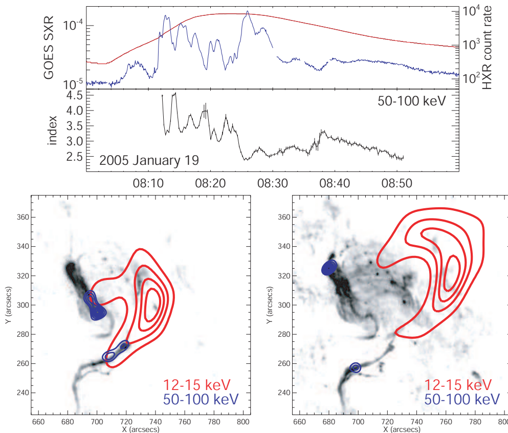
Fig. 8 hard X-ray spectral evolution and imaging of the January 19, 2005 X-class flare (Saldanha et al 2008). Top : the GOES soft X-ray flux (red, low energy channel) and RHESSI 50-100 keV hard X-ray (blue) count rate are shown in the top panel, and the temporal evolution of the power law indices in the energy range between 50 and 100 keV is shown below. Bottom : hard X-ray imaging results of the January 19, 2005 flare taken during the first hard X-ray peaks (08:11:40-08:13:41 UTC, left) with SHS behavior and later during the progressively hardening phase (08:43:10-08:45:40 UTC, right) are presented. Both figures show hard X-ray contours in the thermal (red, contours are 20, 40, 60, and 80 %) and non-thermal (blue, contours levels 7.5, 15, 30, 50, 70, and 90 %) range superposed on TRACE 1600Å images taken at 08:25:30 UTC (first image available for this flare) and 08:45:03 UTC. For both spectral behaviors, soft-hard-soft (SHS) and soft-hard-harder (SHH), non-thermal hard X-ray emissions in the 50-100 keV range are observed from footpoints.
