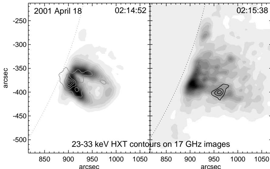
Fig. 6 Contours of hard X-ray emission ( Yohkoh /HXT M1 channel, 23-33 keV) overlaid on 17 GHz images (Nobeyama radioheliograph) at two different times during the extreme behind-the-limb event of 18 April 2001 (Hudson et al 2001). In the first image the radio emission outlines a loop, and the hard X-rays are concentrated just above the limb. In the later image the radio emission is much more diffuse and the hard X-rays originate in a more compact source, well above the limb, that coincides with cool filamentary material seen in the 17 GHz images to move outwards at \approx 1500 \text{ km s}^{-1} for over 5 min, out to a height of 1 R_{\odot} above the limb.
