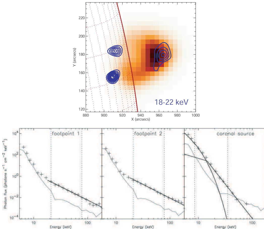
Fig. 11 Imaging spectroscopy with RHESSI. Upper : the July 13, 2005 flare around 14 UTC, showing coronal emission spatially well separated from the hard X-ray footpoints, making it easy to get spectra for the coronal sources and hard X-ray footpoints separately. The RHESSI 18-22 keV contours are averaged over the time period between 14:13:50 and 14:15:48 UTC and overplotted on a GOES SXI image taken at 14:17:05 UTC. Lower : imaging spectroscopy results from Battaglia and Benz (2006).
