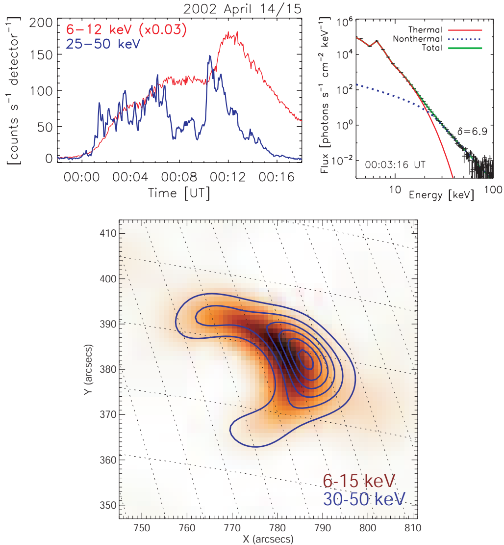
Fig. 4 The coronal thick-target event of 14/15 April 2002: Top : RHESSI light curves and spectrum integrated over the burst at approximately 00:03:30 UTC. Bottom : event-integrated (00:02–00:12 UTC) RHESSI image reconstructed using a MEM (Maximum Entropy Method) algorithm. The color image shows the 6–15 keV thermal image and the blue contours represent the non-thermal emission at 30–50 keV. Contour levels are 20, 35, 50, 65, 80, 95 % of the maximum emission. Most of the non-thermal emission comes from the flare loop, with only a hint of emission from the footpoints.
