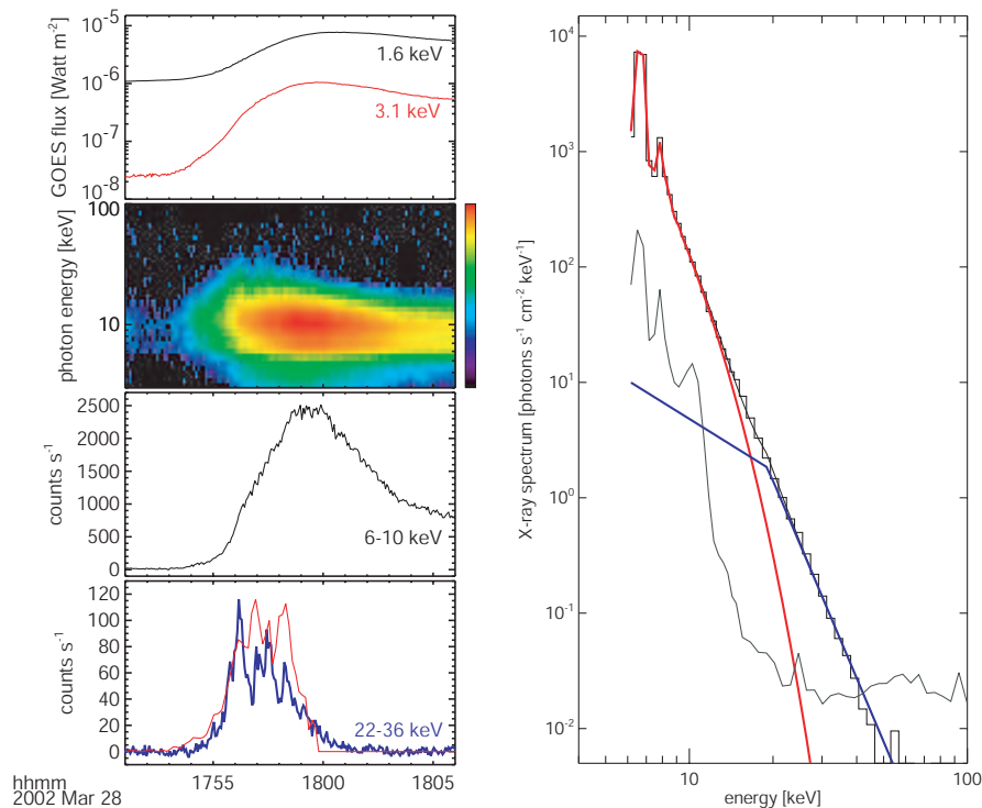
Fig. 12 Typical examples of X-ray time profiles and spectrum of a partially occulted flare (Krucker and Lin 2008). From top to bottom, the panels on the left show GOES soft X-ray time profiles, RHESSI spectrogram plot, time profile of the thermal X-ray emission, and time profile at higher energies (blue). The panels at the bottom additionally show the derivative of the high energy GOES light curve (red) in arbitrary units. The figure on the right shows the X-ray photon spectrum averaged between 17:55:58 and 17:56:18 UTC with a thermal (red, temperature of 24 MK) and non-thermal (blue, \gamma = 5.7 \pm 0.2 ) fit. The gray line represents the background emission.
