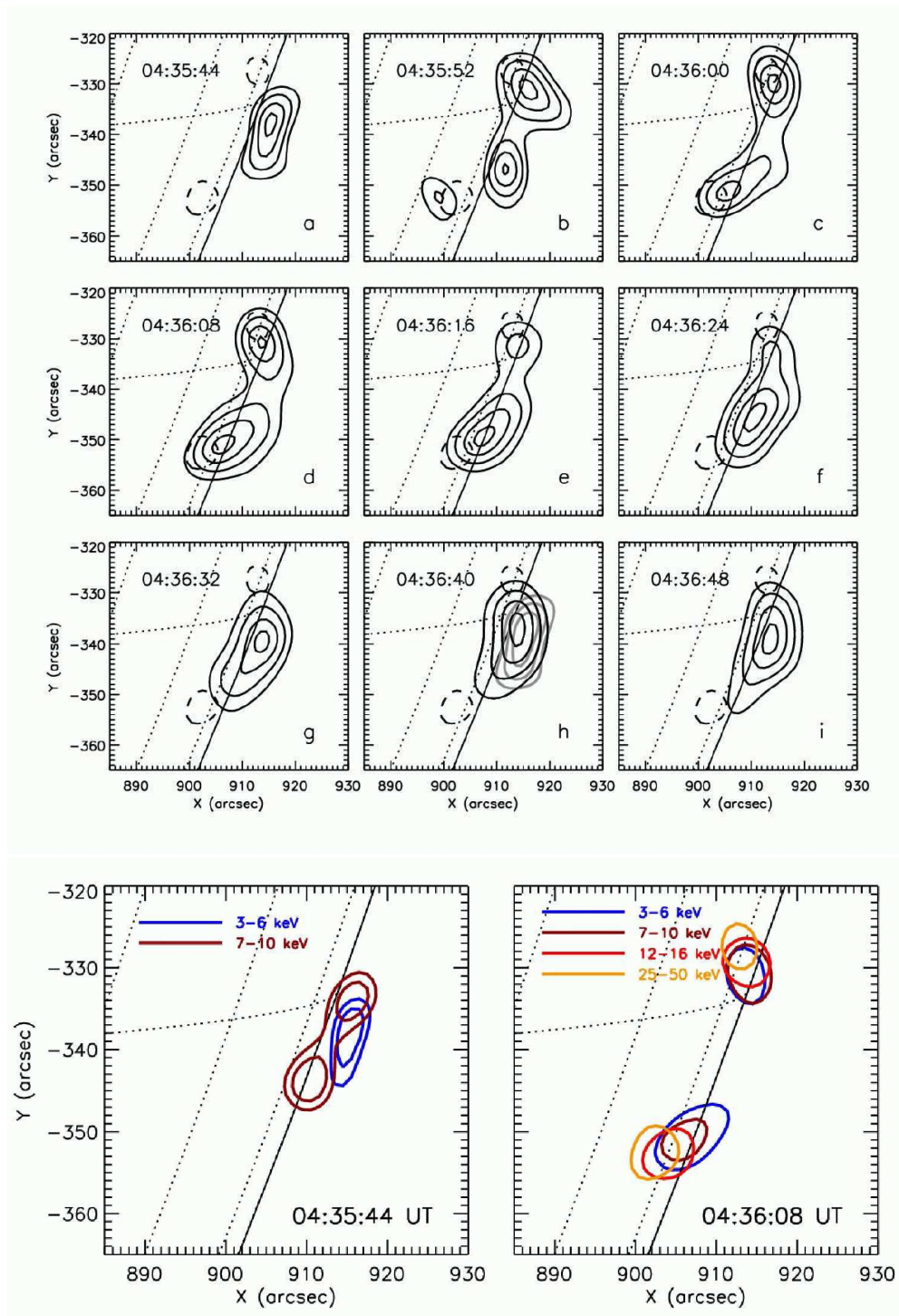
Fig. 5 Upper : RHESSI 3-6 keV maps of the 28 November 2002 flare, showing the apparent motions upwards along a loop; the 25-50 keV contour image (dashed contours) at the hard X-ray peak time is overlaid in each panel. Lower : spectrally-resolved images showing the footpoint locations more clearly. The solid curves in all panels show the solar limb, while the dotted curves show heliographic parallels and meridians.
