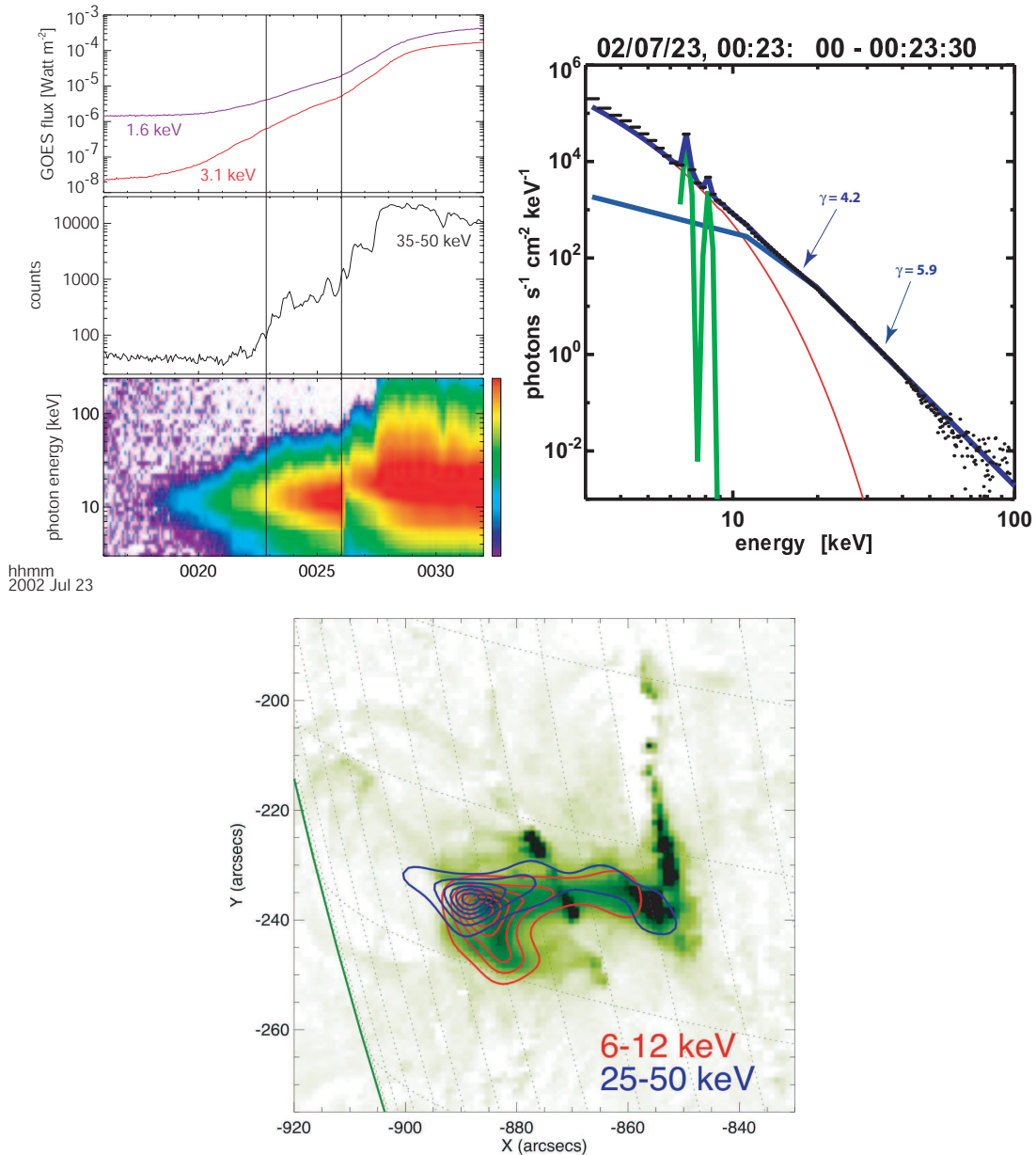
Fig. 1 Example of coronal emission before the impulsive phase in the 23 July 2002 flare. Top left: X-ray time profiles and spectrogram from GOES and RHESSI, showing thermal emission with a gradual evolution and a second component at higher energy with fast time variations of tens of seconds. Top right: Photon spectrum with thermal fit (red) including fits to the Fe and Fe/Ni complexes (Phillips 2004), and non-thermal fit in blue. Bottom: Imaging reveals that the fast time variation component mostly comes from the corona. RHESSI contours in the thermal range (red) and at higher energies (blue) are shown for the time range outlined by vertical bars in the panel to the left. The image shown is a TRACE 195Å image taken at 00:26:00 UTC.
