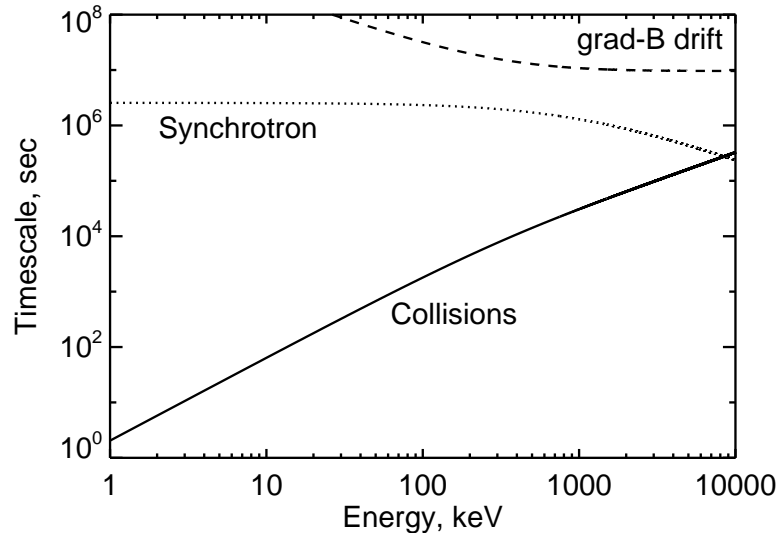
Fig. 16 Representative time scales for fast electrons in the solar corona: solid, the Coulomb collision time assuming a density of 10^8 \text{ cm}^{-3} ; dotted, synchrotron radiation assuming B = 10 \text{ G} ; dashed, gradient-B drift over a spatial scale of 0.1 R_{\odot} .
