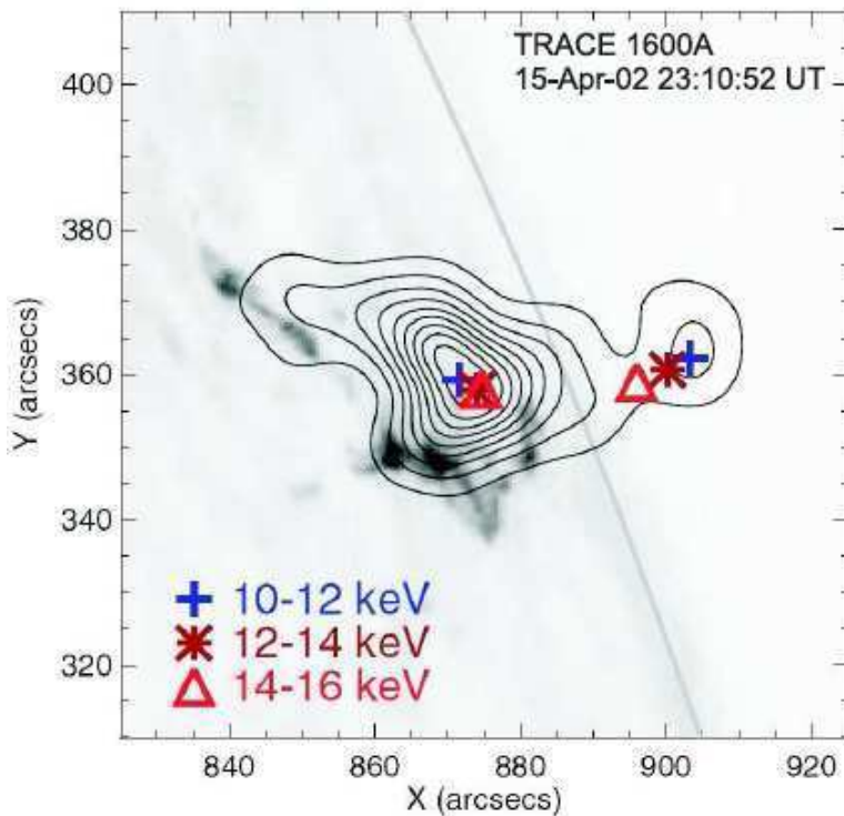
Fig. 3 RHESSI 10–12 keV X-ray image of a flare on 15 April 2002, overlaid on a TRACE 1600 Å filtergram. The RHESSI image shows thermal emission from the flare loops as well as from a source above the loops. The figure shows the emission centroids at three different energies for both the loop-top source and the above-the-loop-top source. The dependence of source height on energy reveals a positive temperature gradient in the lower (loop) source and a negative one in the source above the loops (Sui and Holman 2003).
