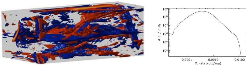
Fig. 14 Left: Snapshot of the resistive electric field configuration inside a coronal loop driven by random motions of the magnetic footpoints at the left and right faces of the simulation box; and right: the distribution function of electric field strength seen by a typical particle traveling inside this “loop.” The red and blue indicate fields pointing towards opposite faces of the box. From Turkmani et al (2006).
