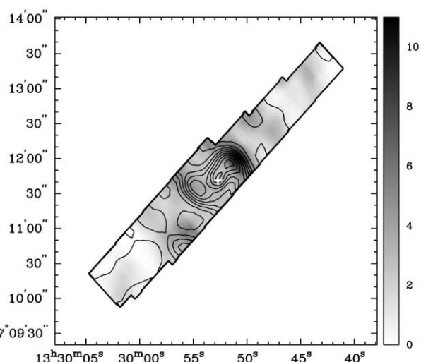
FIG. 8.—Warm ( T = 100\text{--}300 K) \text{H}_2 surface density (in gray scale) compared to the hot ( T = 400\text{--}1000 K) \text{H}_2 surface density (in contours). Contour levels for the hot \text{H}_2 surface density distribution are at intervals of 10% of the maximum surface density ( 0.25 M_\odot \text{pc}^{-2} ). The gray scale is in units of M_\odot \text{pc}^{-2} .
