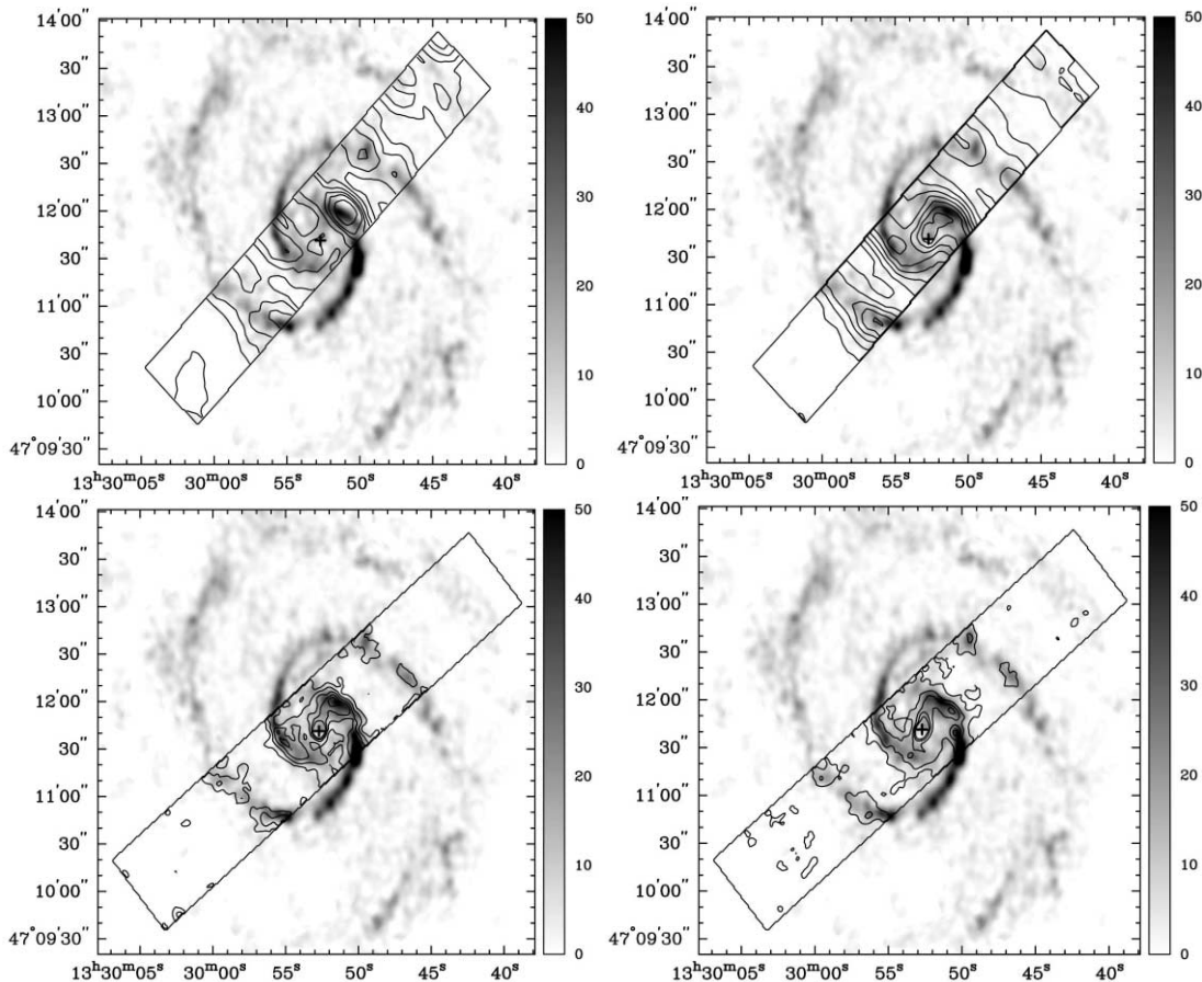
FIG. 10.—Comparison of the CO emission to the \text{H}_2 S(0) (top left), \text{H}_2 S(1) (top right), \text{H}_2 S(2) (bottom left), and \text{H}_2 S(3) (bottom right) emission. The CO emission maps are in units of \text{Jy km s}^{-1} . Contour levels for \text{H}_2 S(0) , \text{H}_2 S(1) , \text{H}_2 S(2) , and \text{H}_2 S(3) are the same as in Fig. 3.
