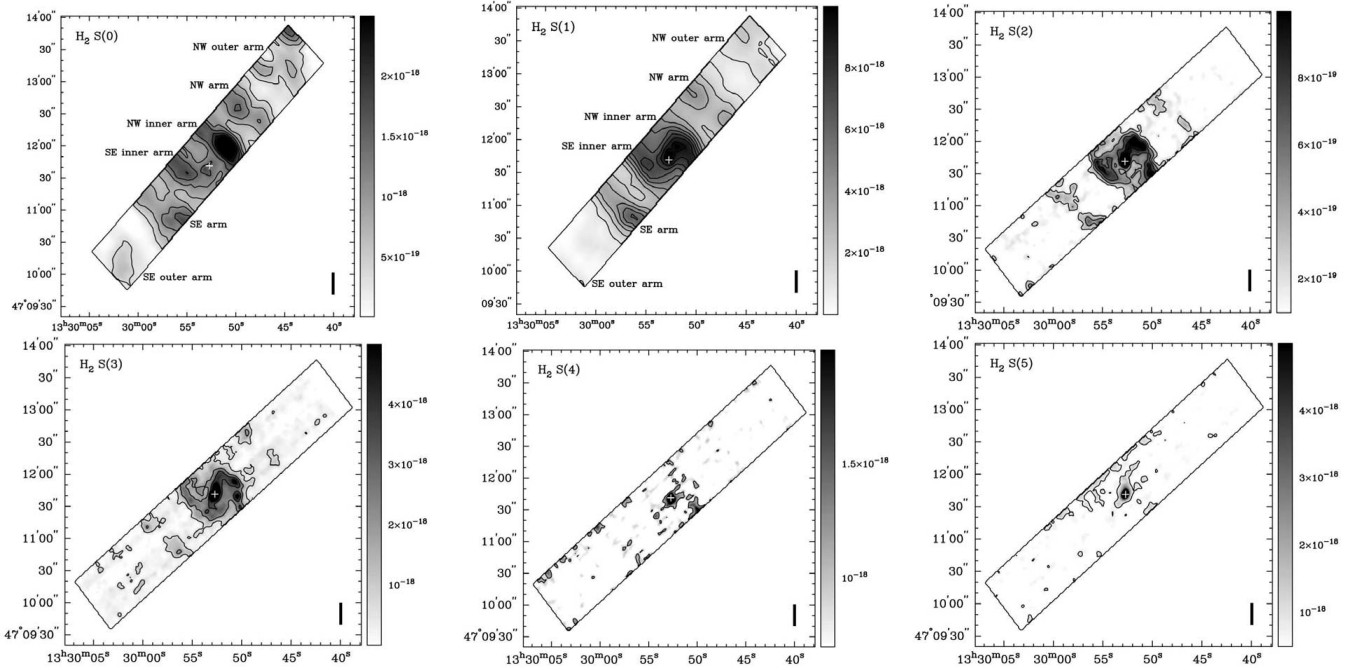
FIG. 3.—Maps of the H_2 S(0) (top left), H_2 S(1) (top middle), H_2 S(2) (top right), H_2 S(3) (bottom left), H_2 S(4) (bottom middle), and H_2 S(5) (bottom right) line fluxes across the SL and LL strips that we mapped with the Spitzer IRS. The H_2 S(0) and H_2 S(1) maps are created from the LL data cube. The H_2 S(2) , H_2 S(3) , H_2 S(4) , and H_2 S(5) maps are created from the SL data cube. The gray scale is in units of W m^{-2} . Contour levels are at 3.7 \times 10^{-19} , 7.3 \times 10^{-19} , 1.1 \times 10^{-18} , 1.5 \times 10^{-18} , 1.8 \times 10^{-18} , 2.2 \times 10^{-18} , and 2.9 \times 10^{-18} W m^{-2} for H_2 S(0) ; 1.1 \times 10^{-18} , 2.1 \times 10^{-18} , 3.2 \times 10^{-18} , 4.3 \times 10^{-18} , 5.4 \times 10^{-18} , 6.4 \times 10^{-18} , 7.5 \times 10^{-18} , 8.6 \times 10^{-18} , and 9.6 \times 10^{-18} W m^{-2} for H_2 S(1) ; 2.2 \times 10^{-19} , 4.4 \times 10^{-19} , 6.7 \times 10^{-19} , 8.9 \times 10^{-19} , and 1.1 \times 10^{-18} W m^{-2} for H_2 S(2) ; 1.3 \times 10^{-18} , 4.0 \times 10^{-18} , 6.7 \times 10^{-18} , 9.4 \times 10^{-18} , and 1.2 \times 10^{-17} W m^{-2} for H_2 S(3) ; 1.0 \times 10^{-18} and 2.0 \times 10^{-18} W m^{-2} for H_2 S(4) ; and 8.0 \times 10^{-19} , 4.0 \times 10^{-18} , and 7.3 \times 10^{-18} W m^{-2} for H_2 S(5) . The vertical axis is the right ascension and the horizontal axis is the declination. In all of the maps, north is up, east is to the left, and the plus sign denotes the nucleus of the galaxy. The different spiral arm regions are labeled on the H_2 S(0) and H_2 S(1) maps in order to aid in discussing the molecular gas morphologies. The bar in the bottom right corner of each map represents 1 kpc. The box around each map represents the SL or LL strip that we mapped.
