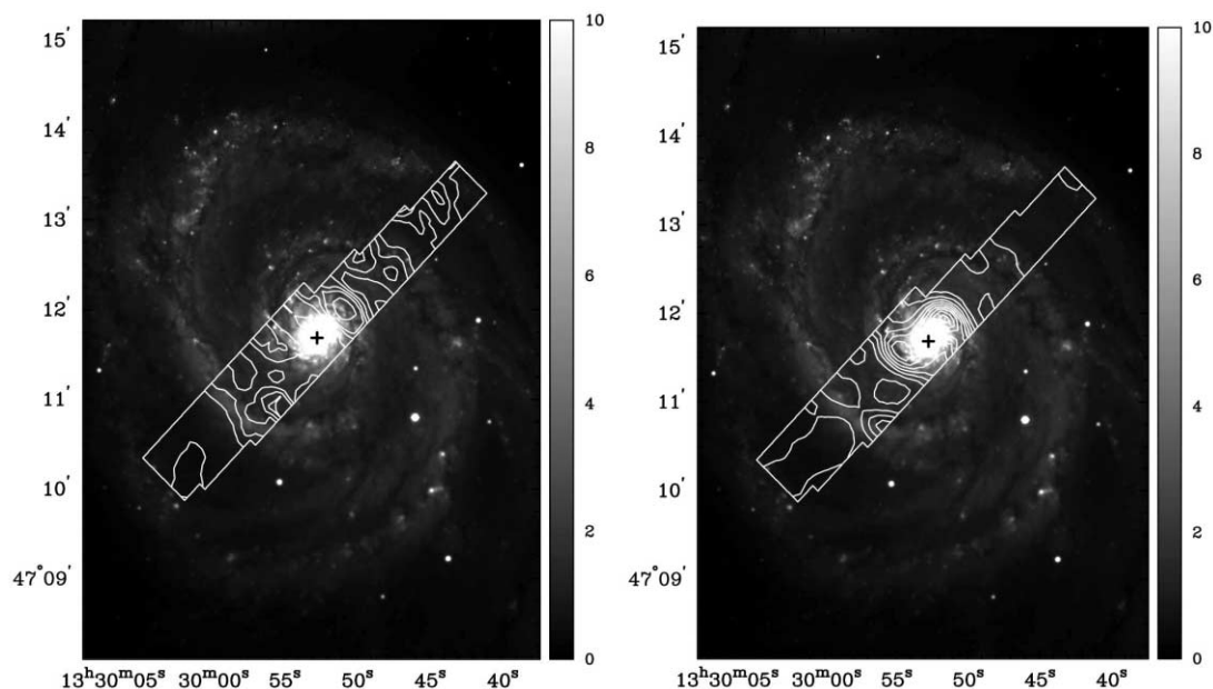
FIG. 12.— Left : Comparison of the V -band image (in gray scale) to the warm ( T = 100\text{--}300\text{ K} ) H_2 surface density (in contours). The V band shows the dust lanes within M51. The V -band image is in units of counts s^{-1} . The warm H_2 surface density contours are the same as in Figs. 5 and 6. Right : Comparison of V -band image (in gray scale) to the hot ( T = 400\text{--}1000\text{ K} ) H_2 surface density (in contours). The V -band image is in units of counts s^{-1} . The hot H_2 surface density contours are the same as in Figs. 5 and 7.
