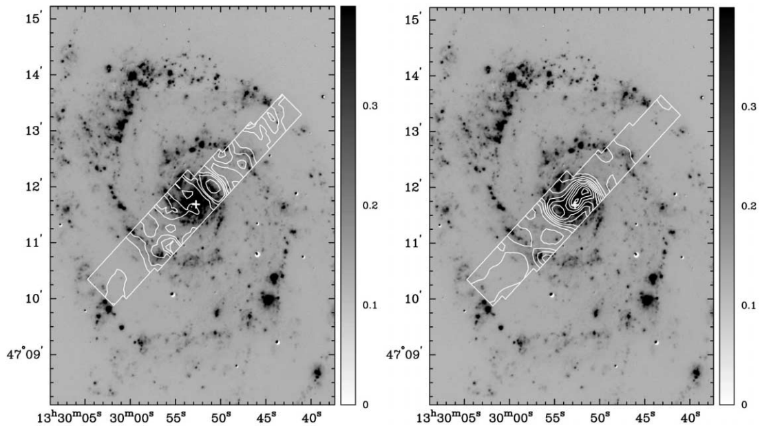
FIG. 11.— Left : Comparison of H\alpha (in gray scale) to the warm ( T = 100\text{--}300\text{ K} ) H_2 surface density (in contours). The H\alpha image is in units of counts s^{-1} . The warm H_2 surface density contours are the same as in Figs. 5 and 6. Right : Comparison of H\alpha (in gray scale) to the hot ( T = 400\text{--}1000\text{ K} ) H_2 surface density (in contours). The H\alpha image is in units of counts s^{-1} . The hot H_2 surface density contours are the same as in Figs. 5 and 7.
