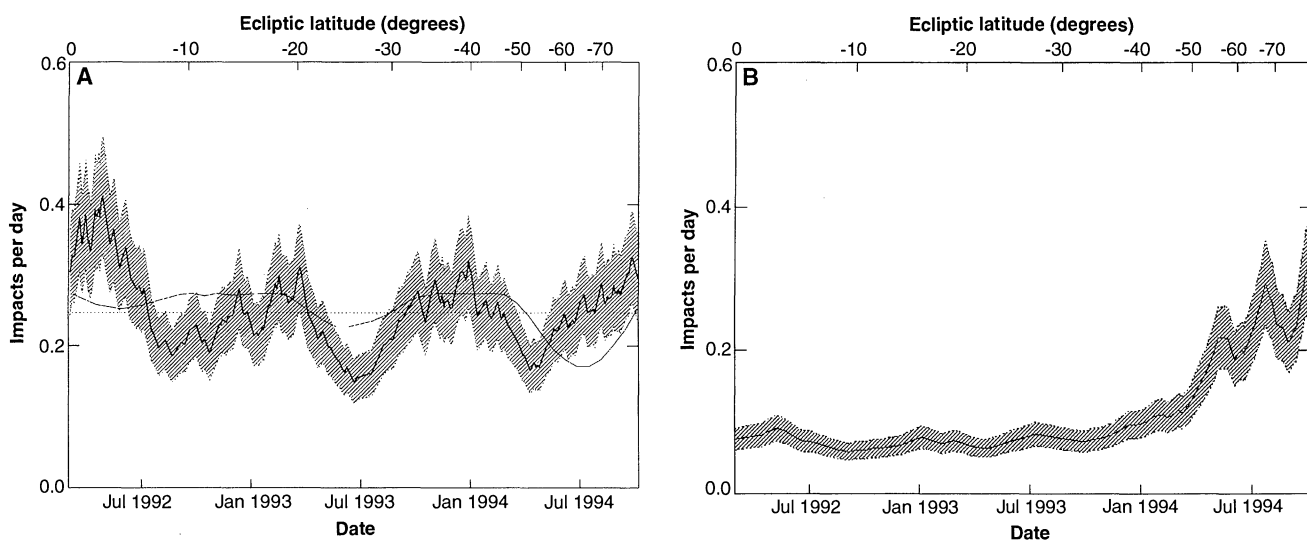
Fig. 3. (A) The impact rates for interstellar grains (thick line). Interstellar grains are identified as nonstream particles compatible with the interstellar direction (Fig. 1B). The rates were calculated with a sliding average over 25 particles; statistical errors are indicated by the hatched region surrounding the impact-rate curve. The dotted line shows the average impact rate of 0.25 impacts per day, and the thin solid line indicates the sensitivity, averaged over a full
