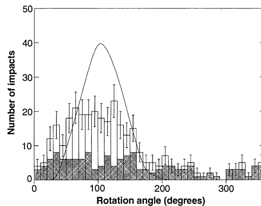
Fig. 2. Number of detections versus rotation angles recorded over the entire 2.5-year period excluding Jupiter stream particles. The number of impacts per 10° rotation angle interval are shown for large particles (white histogram) and for small particles with masses <math>6 \times 10^{-14}</math> g (crosshatched histogram). Error bars are calculated for the sum of small and large particles assuming a \sqrt{n} statistical error. The solid line indicates the distribution expected for particles arriving from the assumed upstream interstellar direction. It is derived by integrating Fig. 1B over time. The slight asymmetry of the curve about its peak is due to slow changes in the orientation of the spacecraft's spin axis.
