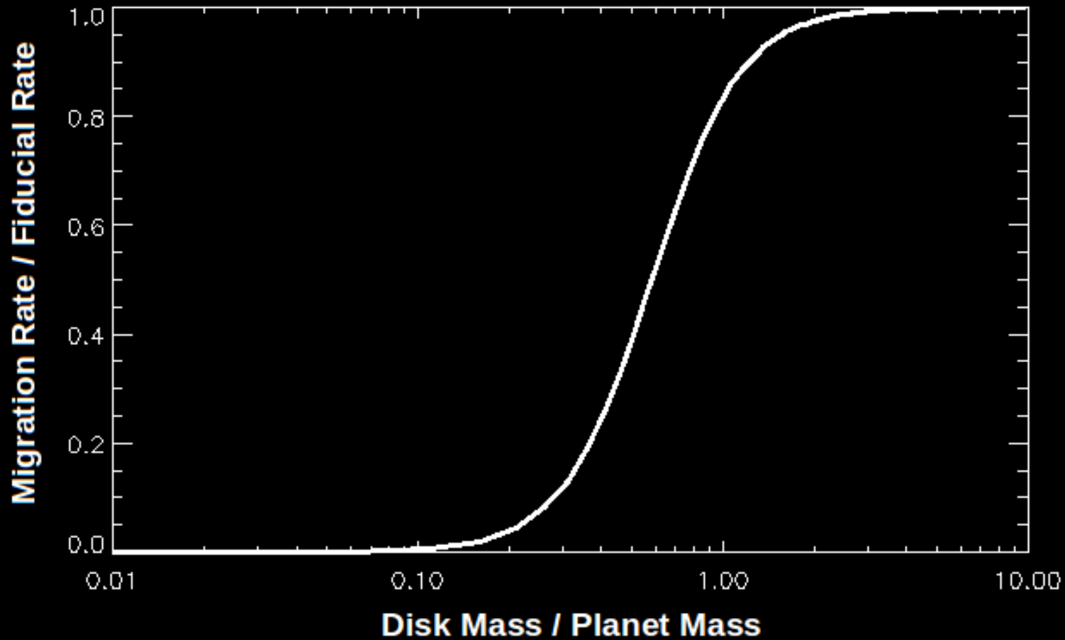
Migration Rate: Disk Mass
