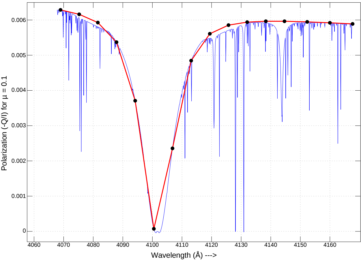
T=12000K, lg=3.5: continuum + H-delta (red) vs all lines (blue)
