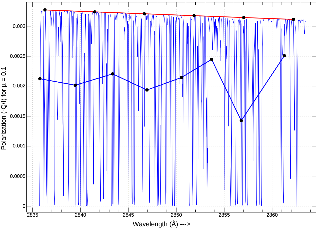
T=12000K, lg=3.5: continuum (red) vs with lines resolved (blue) & averaged (thick)
