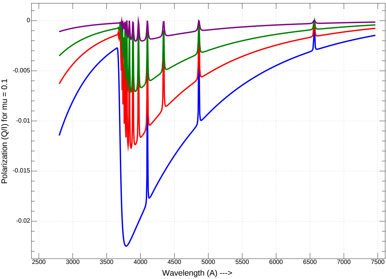
Kurucz models: T=12,000\text{K} , \log g = 2.5, 3.0, 3.5, 4.0
