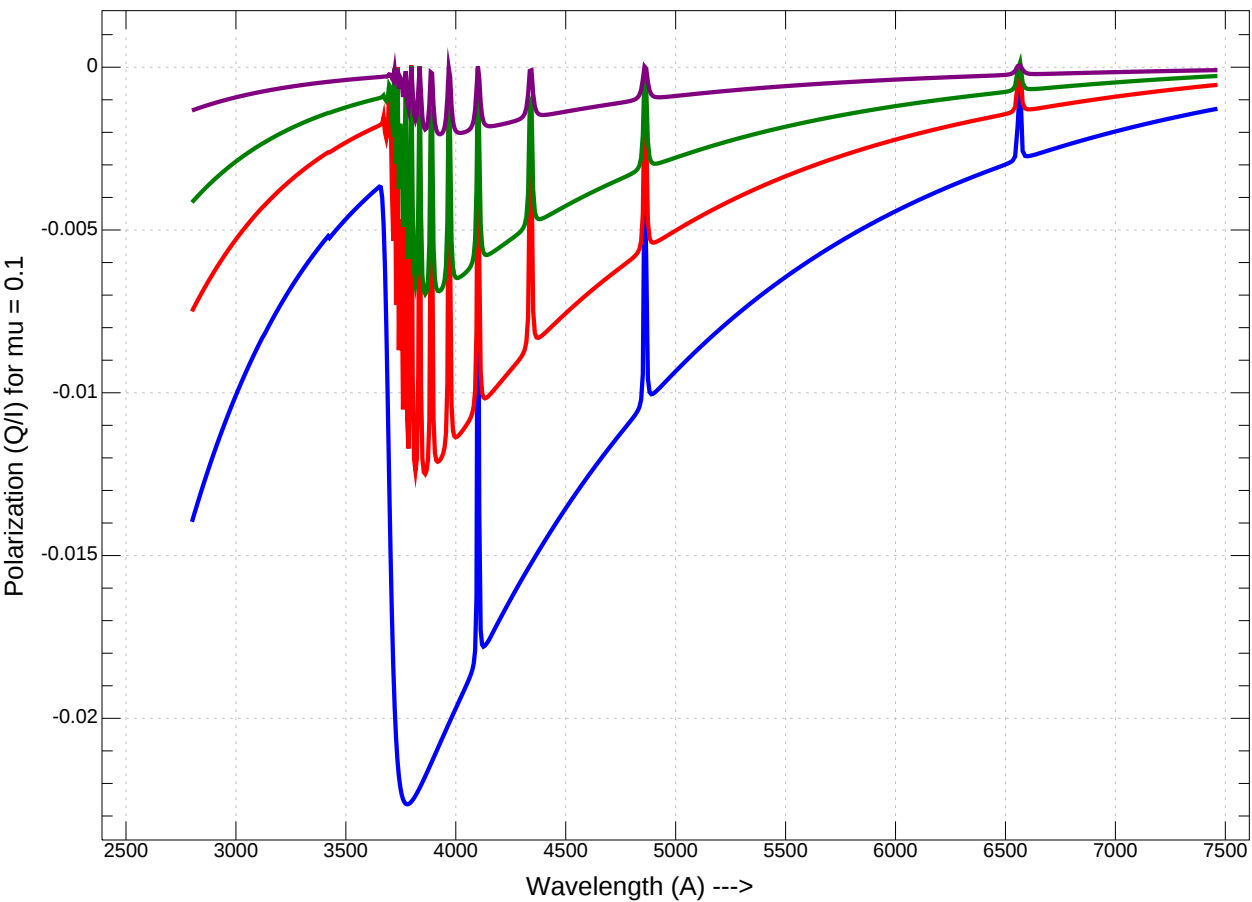
Kurucz models: T=14,000\text{K} , \log g = 2.5, 3.0, 3.5, 4.0
