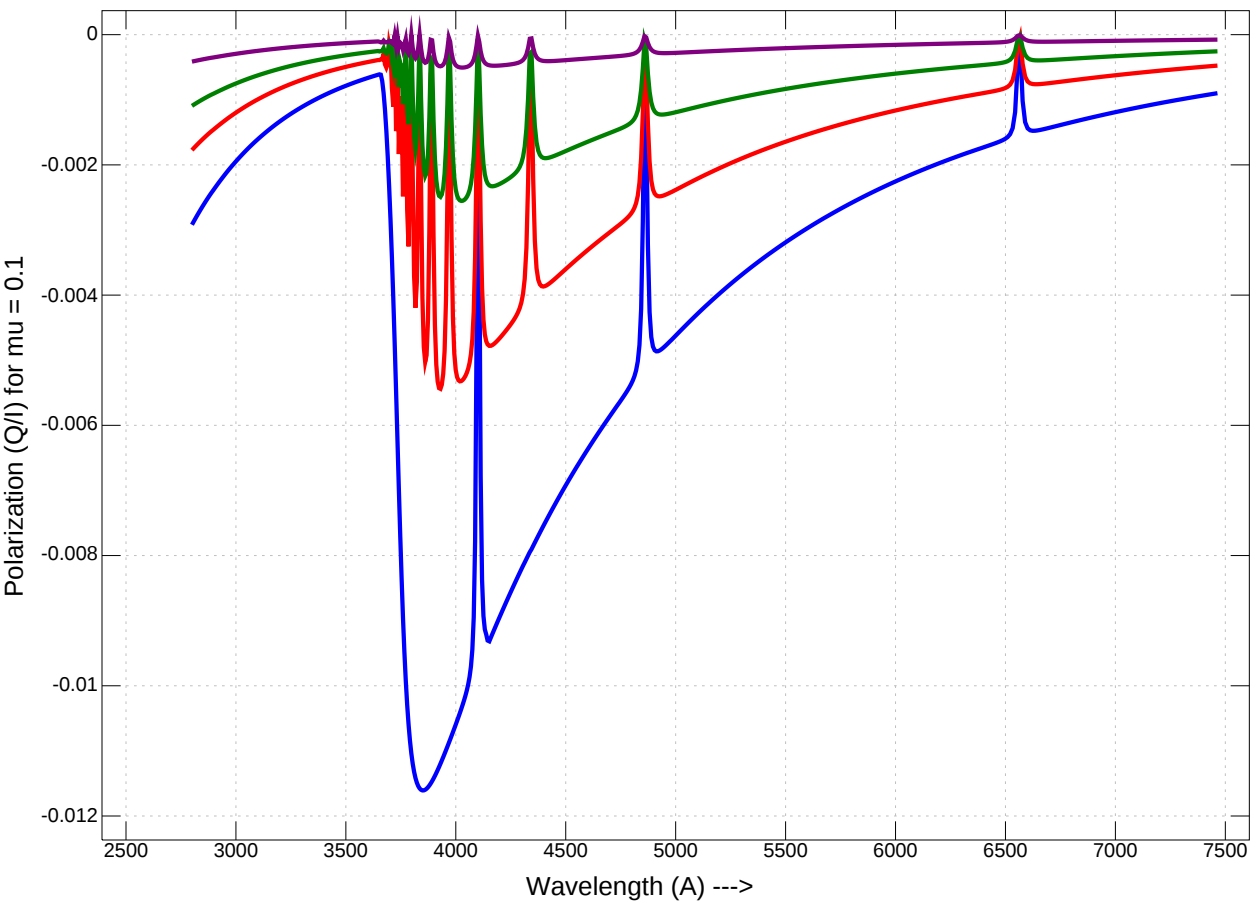
Kurucz models: T=8000\text{K} , \log g = 2.5, 3.0, 3.5, 4.0
