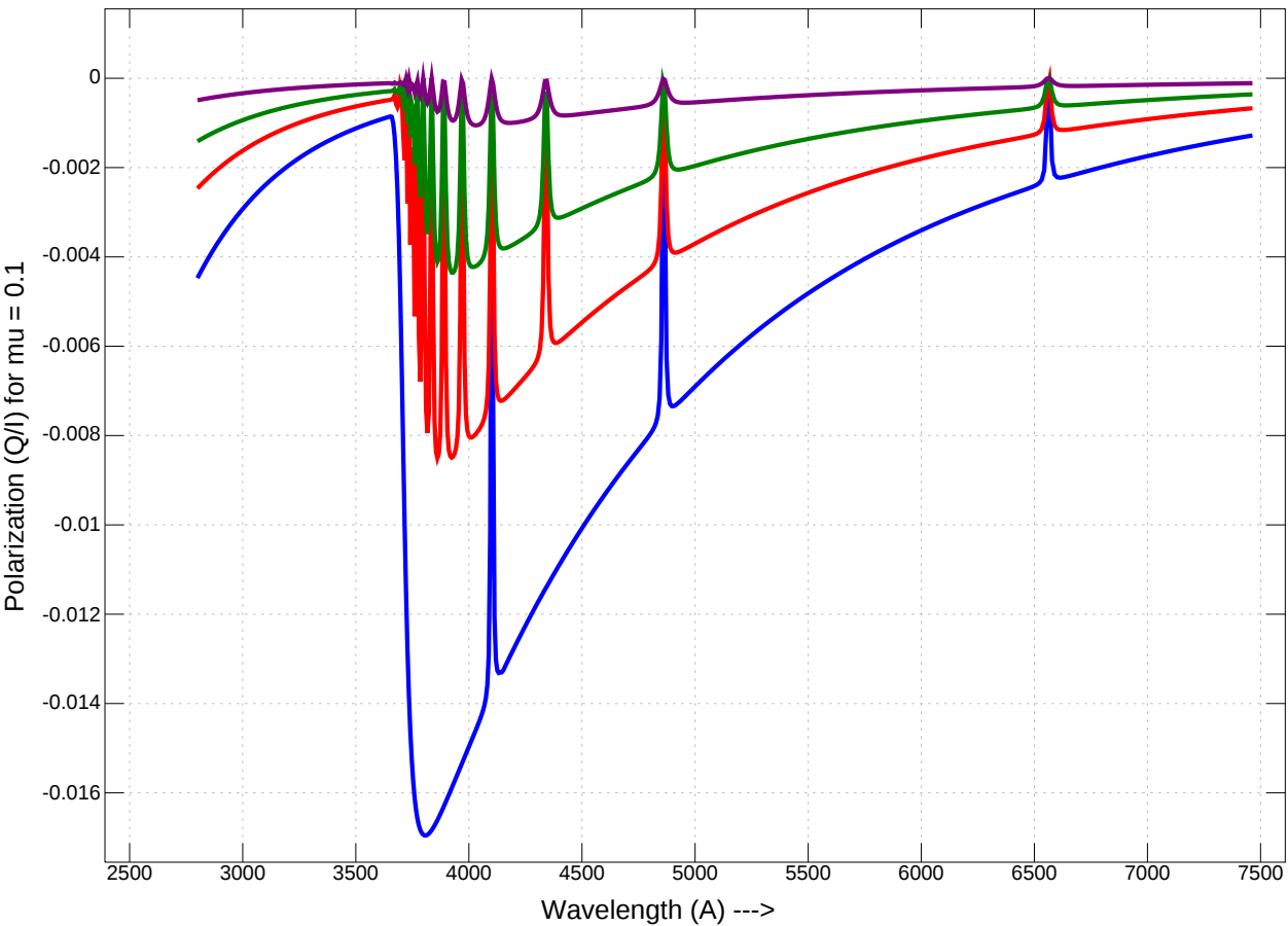
Kurucz models: T=9000\text{K} , \log g = 2.5, 3.0, 3.5, 4.0
