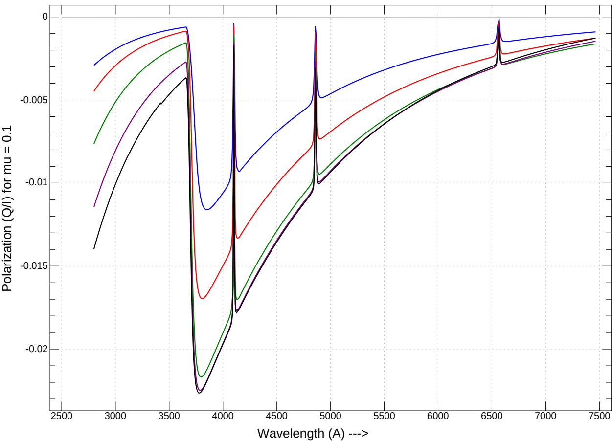
Kurucz models: \log g = 2.5 for T=8000\text{K} , 9000\text{K} , 10,000\text{K} , 12,000\text{K} , 14,000\text{K}
