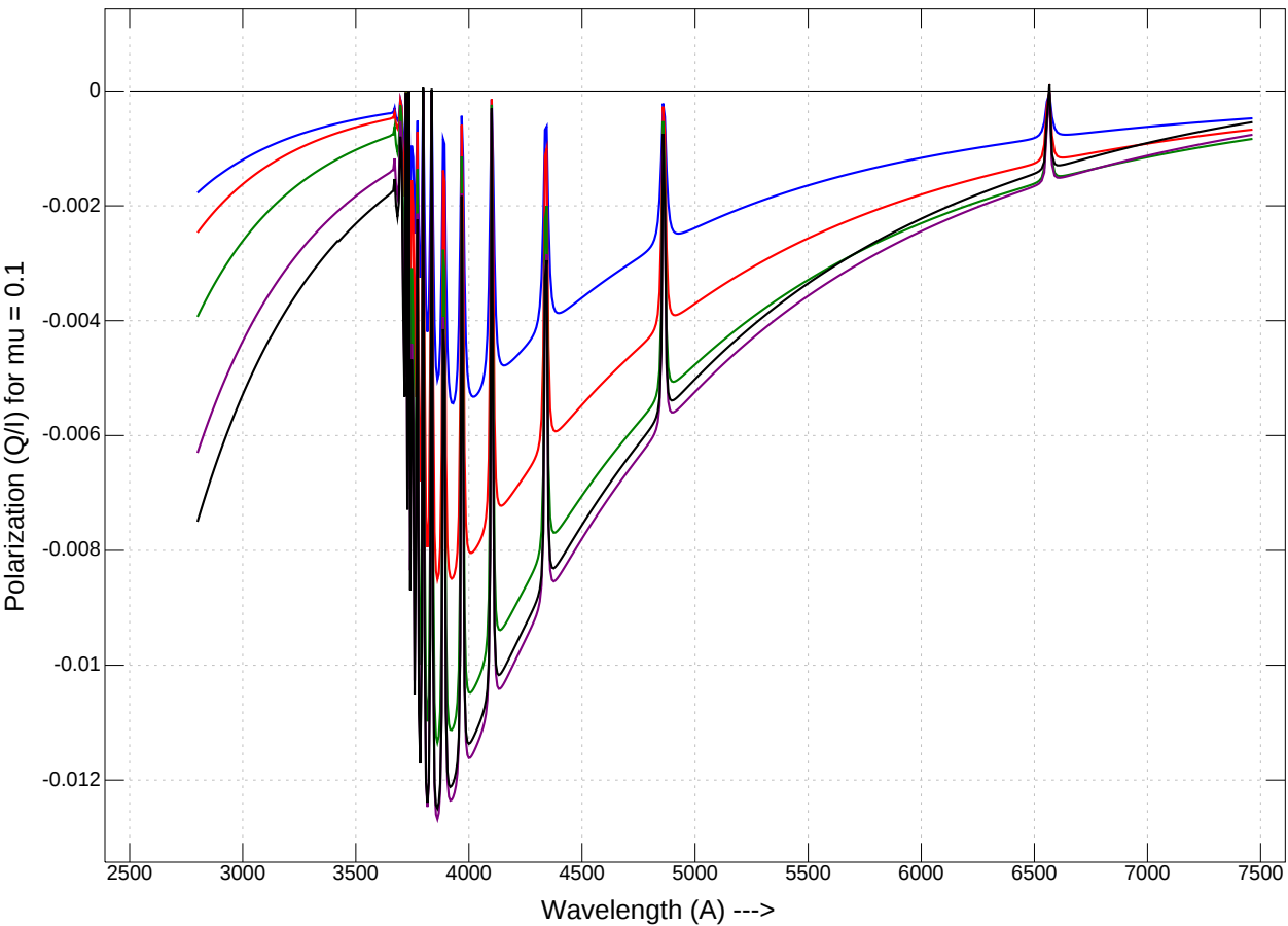
Kurucz models: \log g = 3.0 for T=8000\text{K} , 9000\text{K} , 10,000\text{K} , 12,000\text{K} , 14,000\text{K}
