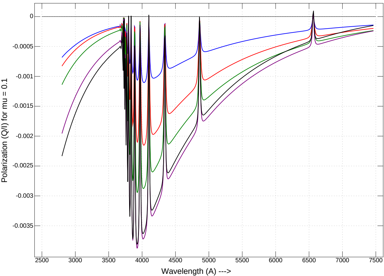
Kurucz models: \log g = 4.0 for T=8000\text{K} , 9000\text{K} , 10,000\text{K} , 12,000\text{K} , 14,000\text{K}
