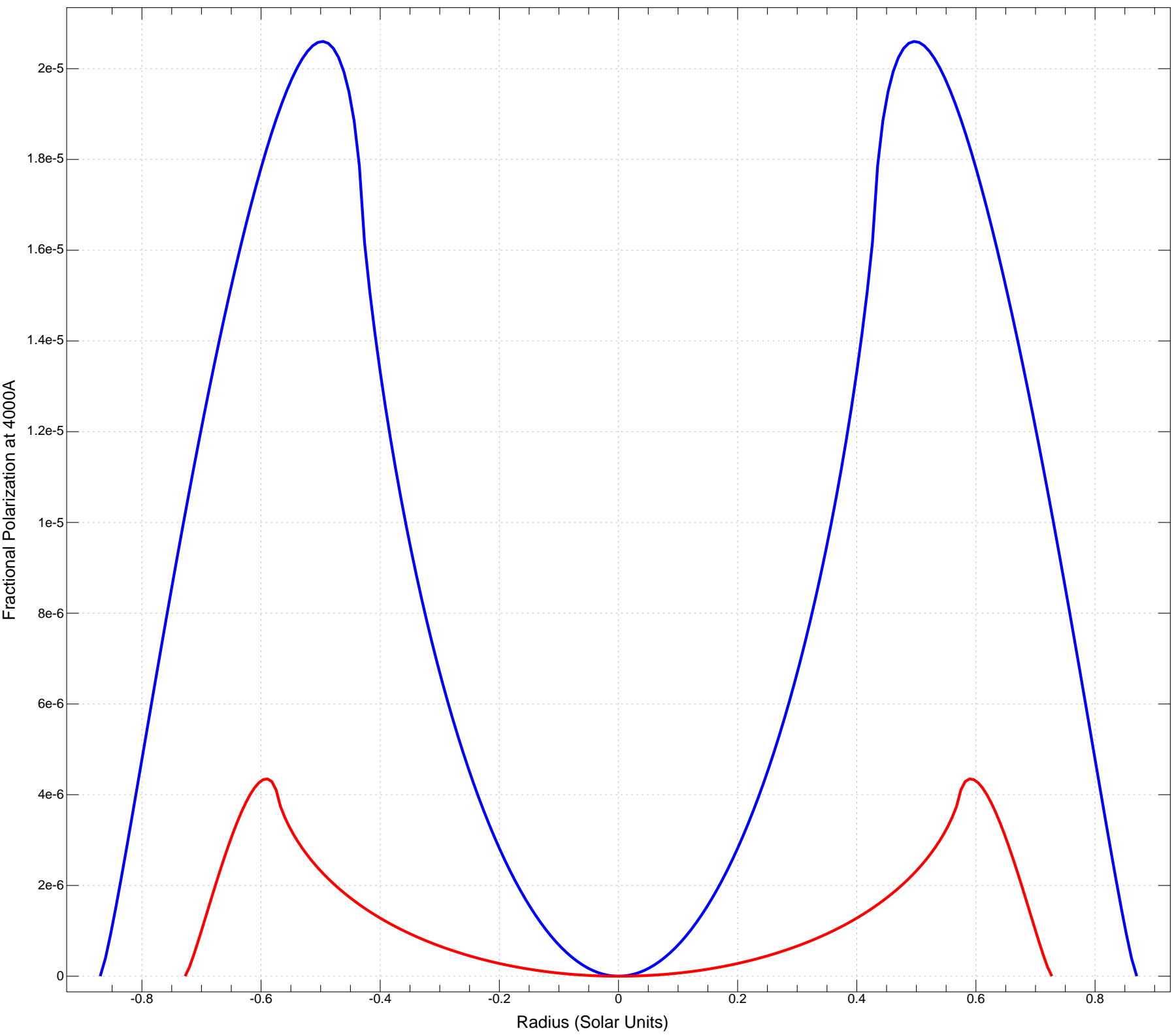
Transit of Kepler-16A by star B(blue) and planet b(red).
