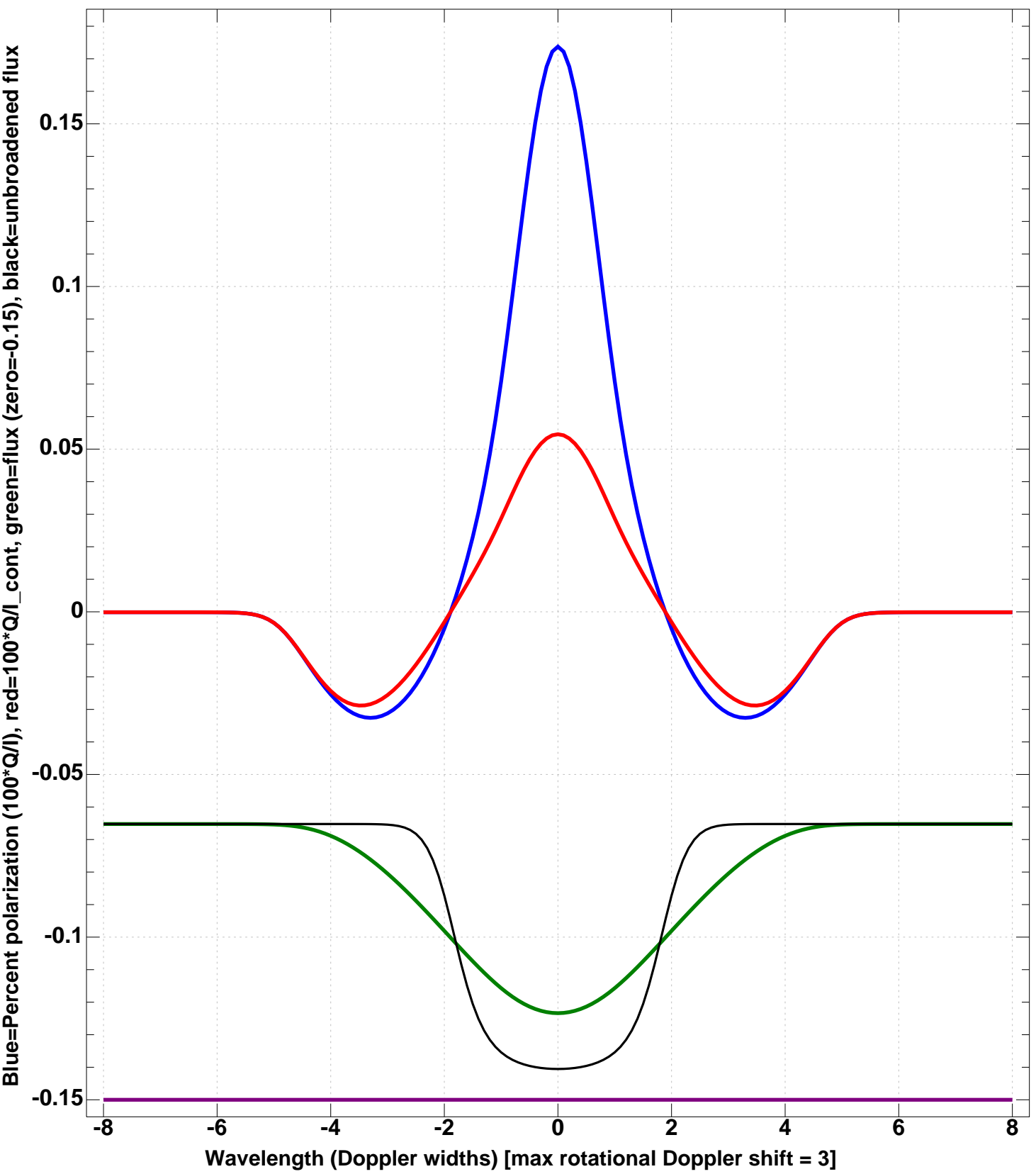
Milne-Eddington \tau(0)=15 line at 4000Å in T=4000K, \lg=3 , MARCS model
