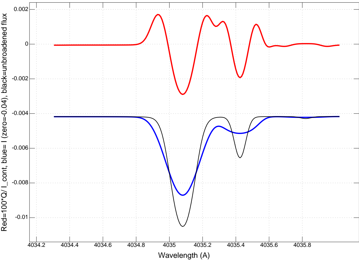
Stokes I&Q across lines of rotating star: T=30,000K, lg=4.0 -- Rot vel = 10 km/s
