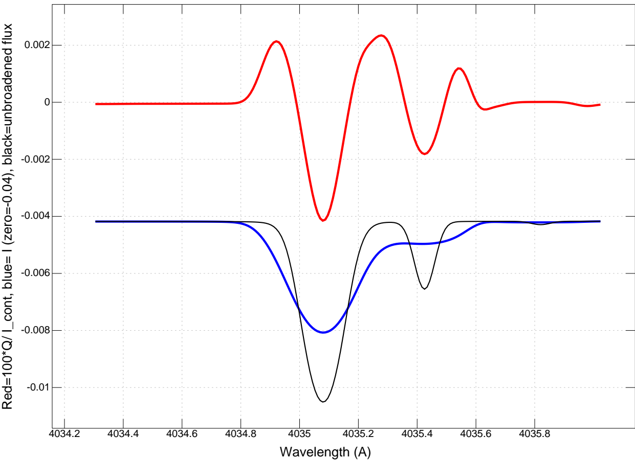
Stokes I&Q across lines of rotating star: T=30,000K, lg=4.0 -- Rot vel = 12.5 km/s
